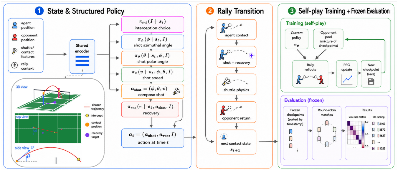
Figure 1: Overview of ShuttleArena, including the state, role-conditioned policy, rally transition, and evaluation pipeline. The policy observes player positions, shuttle/contact features, feasible interception information, and rally context. On receiver turns it selects a feasible interception candidate; after contact, on hitter turns it factorizes the outgoing action into shot azimuth, elevation, speed, and recovery. The left panel compactly shows these consecutive decisions in one receive-and-return chain; they are not sampled jointly in one simulator step. ShuttleArena advances the rally through shuttle physics and opponent response, while PPO self-play trains against a checkpoint mixture and frozen checkpoints are evaluated by round-robin win-rate and rating analyses.
