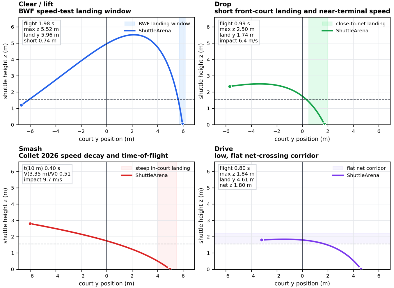
Figure 10: Shuttle trajectory validation for four canonical shot families. Each panel shows the side-view ShuttleArena trajectory under the paper’s drag-square parameters ( k_h = 0.20 , k_v = 0.16 ). Shaded regions indicate external or canonical reference bands: the BWF correct-speed clear/lift landing window, close-to-net drop landing, Collet’s smash flight-time and speed-decay range, and a low drive net-crossing corridor. These checks are intended as plausibility validation of the shuttle-flight model, not as detailed calibration of player biomechanics or racket contact.
