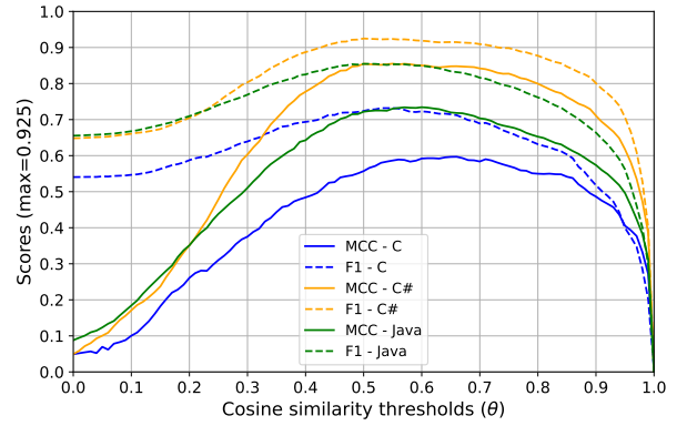
Fig. 4: Scores across \theta using Python-trained LWVIC4Code.
