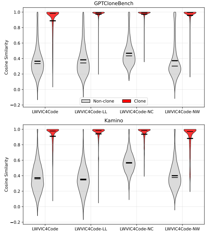
Fig. 3: Cosine similarity distributions of clone and non-clone pairs for LWVIC4Code variants.
