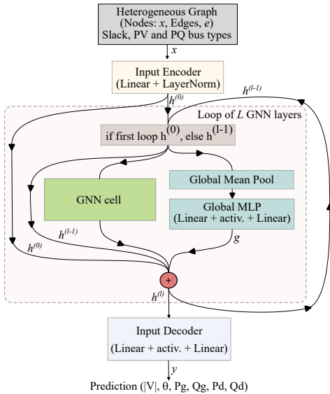
Fig. 3. Architecture of the proposed unified Heterogeneous ResGated GCN.
