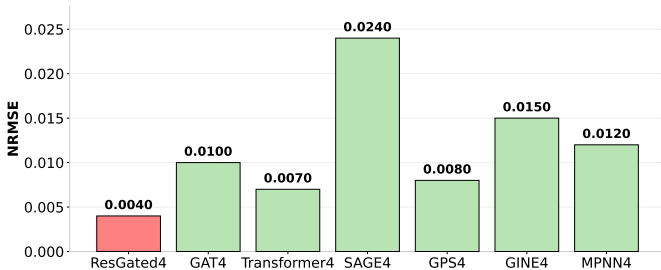
Fig. 4. GNN cell comparison showing average NRMSE.
