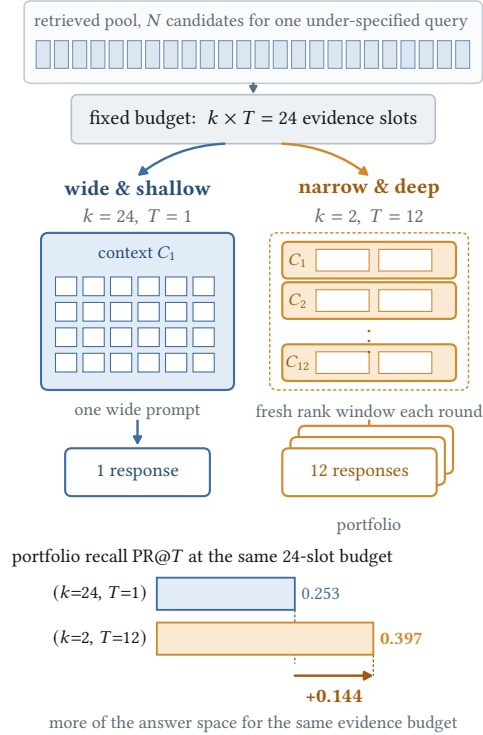
Fig. 1. The context-allocation problem in one picture. (a) A fixed inference budget of k \times T evidence slots can be packaged as one wide context ( k=24, T=1 ) or as many narrow contexts that rotate through fresh evidence ( k=2, T=12 ). Both consume 24 retrieved documents, yet the second packaging covers +0.144 more of the answer space (Table 4). (b) Turning that allocation law into a scheduler: on a frozen held-out frame, Ascp beats every selection-style baseline by +0.033 to +0.081 portfolio recall (all BH q < .001 ); the two grey arms are reference configurations whose remaining gaps are not significant (Table 10). (c) None of this is measurable with relevance proxies. Swapping the padding of the evaluation pool from off-query distractors to same-query hard negatives that entail no answer leaves the causal leave-one-out probes almost unchanged ( -0.01 AUC), while BM25 and query-document cosine fall by more than 0.5 to chance (Figure 3).
