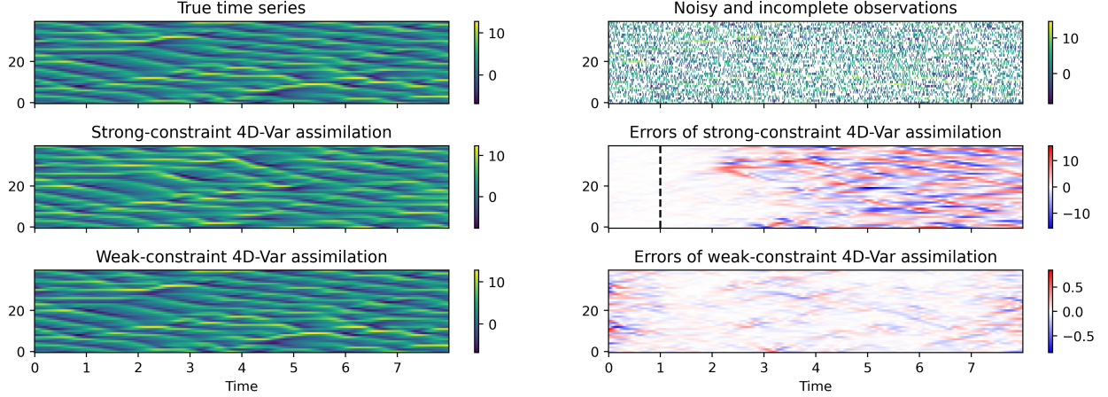
Figure 4: Visualization of the true state values, the corresponding sparse and noisy observations, and the state estimations and errors obtained by strong- and weak-constraint 4D-Var on the Lorenz-96 dynamical system. The dashed vertical line marks the limit of assimilated observations for strong-constraint 4D-Var.
