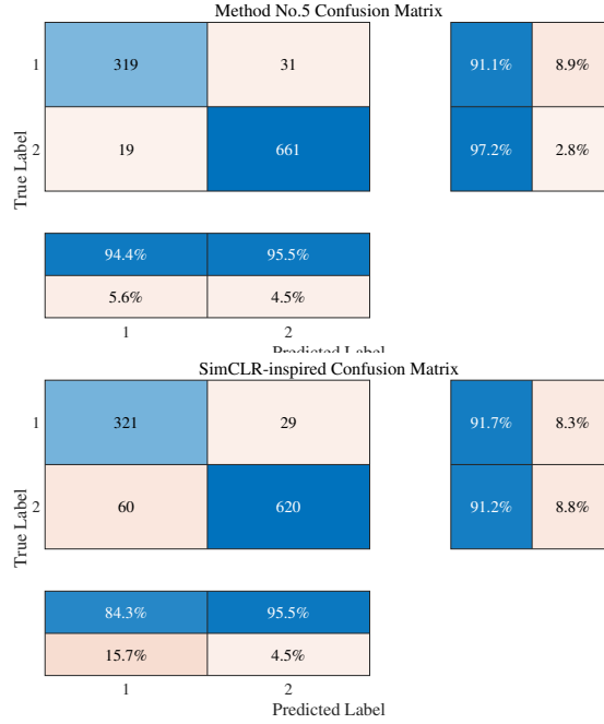
Figure 4: The confusion matrices of KLPCDA Method No.5 and SimCLR-inspired baselines on GSE44076 colon cancer dataset.
