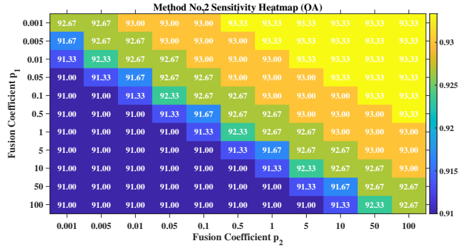
Figure 6: The fusion coefficient parameter sensitivity heatmap of Method No.2 on GSE44076.
