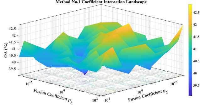
Figure 5: The fusion coefficient parameter sensitivity surface of Method No.1 on Indian Pines.
