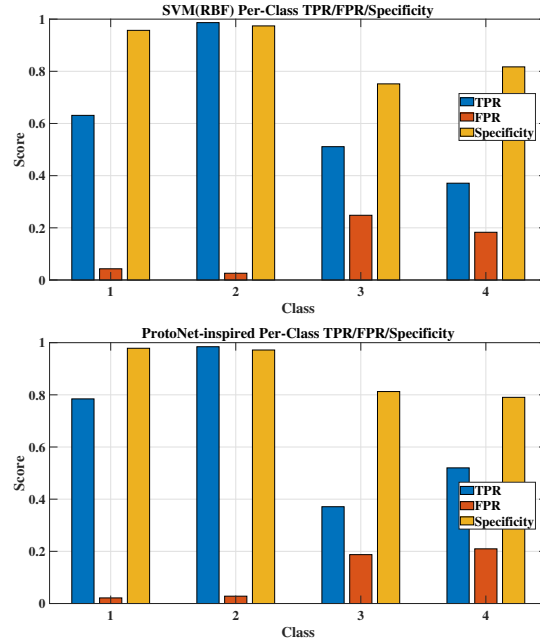
Figure 3: The per-class TPR, FPR, and specificity of the SVM and ProtoNet-inspired baselines on CWRU.
