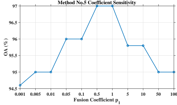
Figure 7: The fusion coefficient parameter sensitivity of Method No.5 on JAFFE Identity Recognition.
