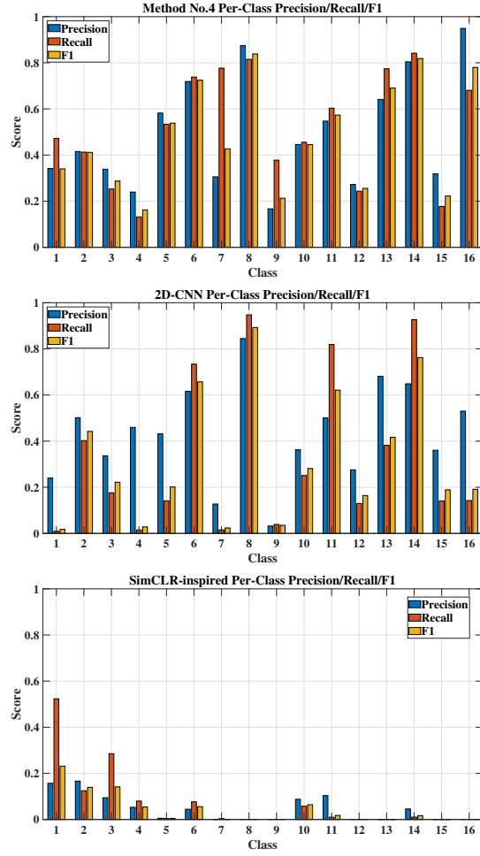
Figure 1: The per-class precision, recall, and F1-score of KLPCDA Method No.4, 2D-CNN and the SimCLR-inspired baseline on Indian Pines.
