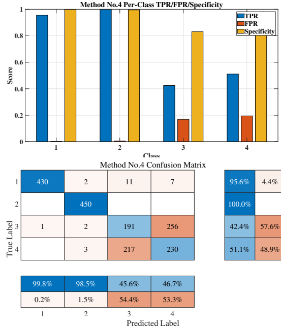
Figure 2: The per-class TPR, FPR, and specificity and the confusion matrix of KLPCDA Method No.4 on CWRU.
