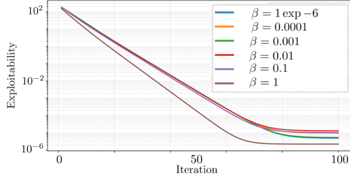
FIGURE 3. Exploitability for Stock Market Trading.
