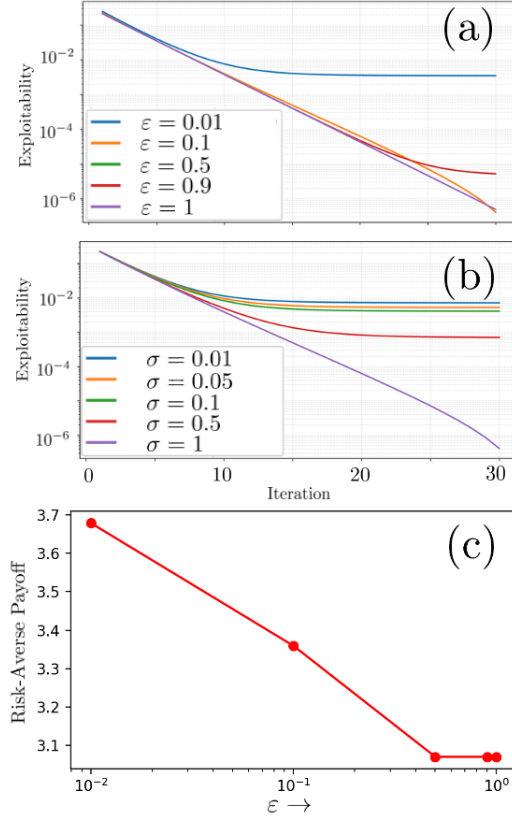
FIGURE 4. (a) Varying \epsilon under \sigma = 1 ; (b) Varying \sigma under \epsilon = 0.1 ; (c) Cumulative rewards.
