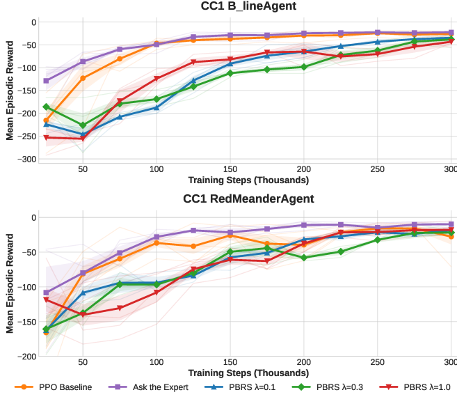
Fig. 2. Mean checkpoint evaluation reward for PPO, Ask the Expert , and PBRS variants in CC1. Top: B_lineAgent. Bottom: RedMeanderAgent. Shaded bands denote \pm 1 standard error across independent training seeds.
