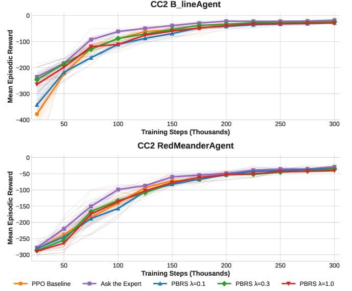
Fig. 3. Mean checkpoint evaluation reward for PPO, Ask the Expert , and PBRS variants in CC2. Top: B_lineAgent. Bottom: RedMeanderAgent. Shaded bands denote \pm 1 standard error across independent training seeds.
