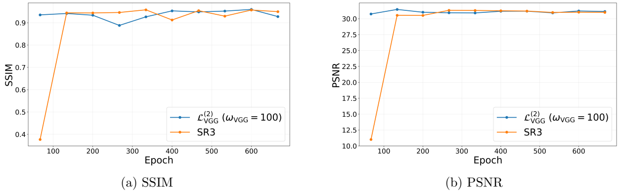
Figure 5: Convergence comparison between the proposed method ( \mathcal{L}_{\text{VGG}}^{(2)} , \omega_{\text{VGG}} = 100 ; blue) and the baseline SR3 model (orange) on the BrainWeb 2\times task in terms of SSIM (left) and PSNR (right). The proposed method converges faster than SR3 and the two methods eventually reach similar SSIM and PSNR.
