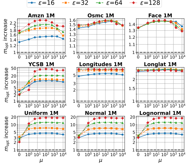
Figure 18: Effect of \mu on m_{\text{opt}} for \lambda = 100,000 .
