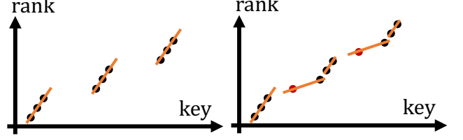
Figure 14: An example of the tight upper bound (Theorem 6), where \lambda = 2 and \varepsilon = 0 . Before poisoning (left), m_{\text{opt}}(\mathcal{K}, \varepsilon) = 3 and after poisoning (right), m_{\text{opt}}(\mathcal{K} \cup \mathcal{P}, \varepsilon) = 5 .
