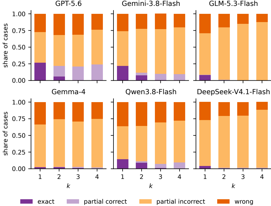
Figure 12: Interactive outcomes by k (DDXPlus, 200 cases per k ). A partially correct set is a subset of the truth; a partially incorrect one adds wrong labels.
