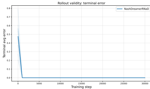
Figure 19: Rollout terminal-flag error in Goofspiel-5, at zero within 1,000 gradient steps.
