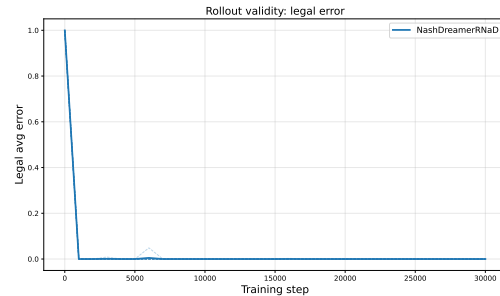
Figure 20: Rollout legal-action-mask error in Goofspiel-5, likewise at zero within 1,000 gradient steps.
