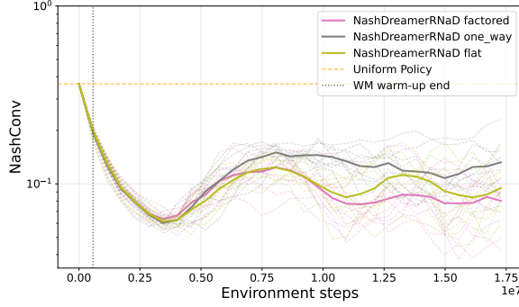
Figure 6: NashConv in Leduc Poker for the three latent and loss configurations of NashDreamer[RNaD]: the factored latent, the flat single-categorical latent, and the one-way variant with \beta^{\text{enc}} = 0 . All three deteriorate after the initial descent, the one-way variant furthest and the factored latent least. Bold curves are means over the 10 training seeds, faint curves the individual seeds; the dotted line marks the end of the world-model warm-up.
