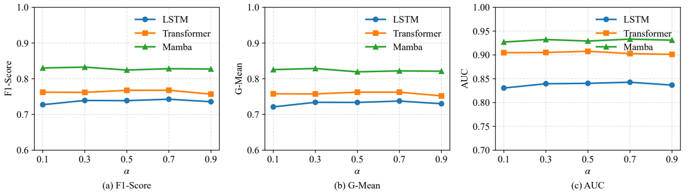
Fig. 7. Sensitivity analysis of the trade-off coefficient \alpha in the Stage-II fitness function.
