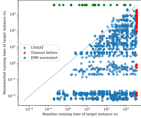
(a) Warmstart for different \varepsilon on UNSAT source and UNSAT or TIMEOUT target instances.
