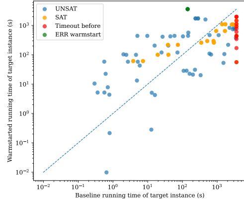
(d) Warmstart for the same \varepsilon and image, but different networks as source and target instances.
