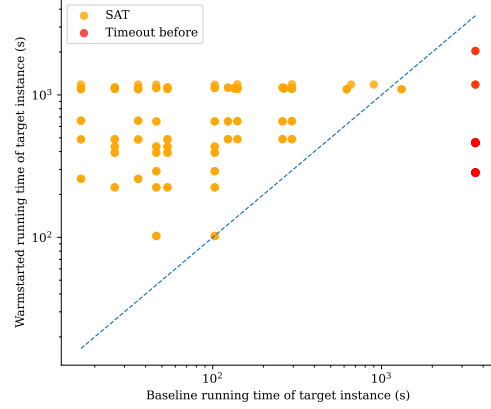
(b) Warmstart for different \varepsilon on SAT source and SAT or TIMEOUT target instances.
