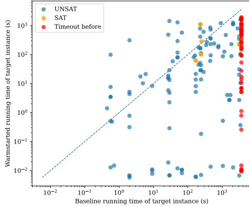
(c) Warmstart for the same \varepsilon and network, but different images as source and target instances.
