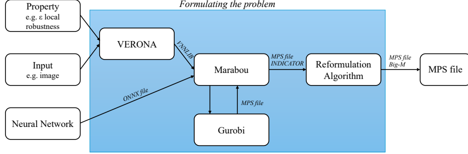
Figure 1: The pipeline created to formulate the verification tasks as MPS files that can be used as inputs for the SYMPHONY solver.
