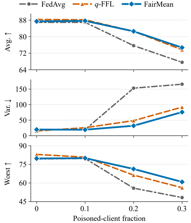
Fig. 2. Fashion-MNIST performance under pairwise flip versus the poisoned-client fraction.
