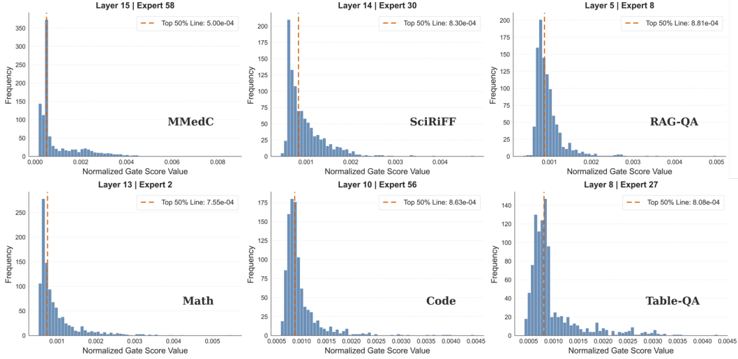
Figure 5: Intra-expert activation sparsity across domains. Each subplot shows the normalized channel-wise gate-score distribution of a representative OLMoE expert. The dashed orange line marks the top-50% cumulative activation threshold. The strong concentration near zero across domains indicates that only a small subset of channels is highly activated inside selected experts.
