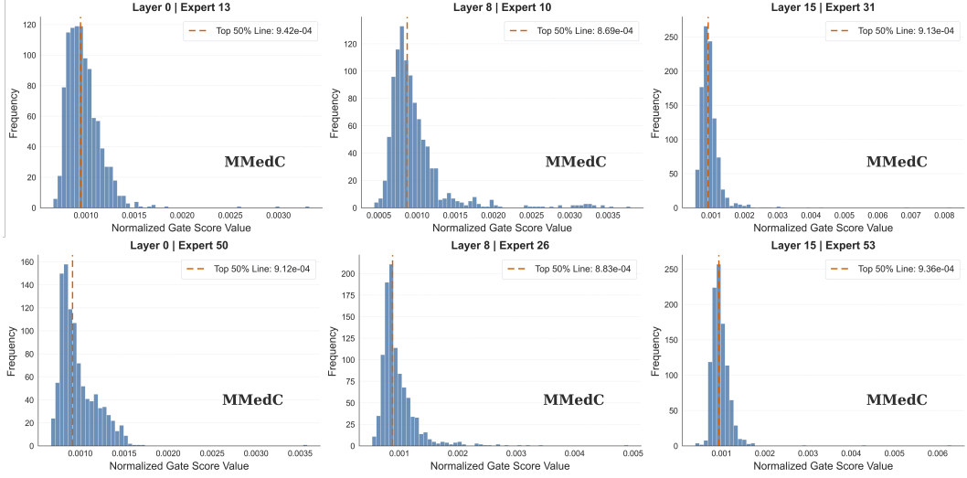
Figure 6: Channel-wise gate-score distributions for randomly sampled experts from shallow, middle, and deep layers on MMedC, with two experts sampled from each depth range. The dashed orange line marks the threshold covering the top 50% cumulative activation mass.
