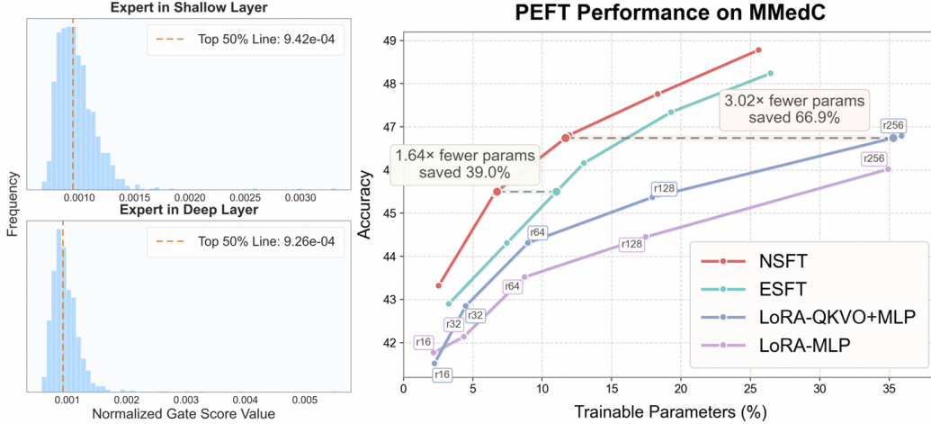
Figure 1: Left: channel-level gate-score distributions of shallow and deep OLMoE experts on MMedC, showing strong intra-expert sparsity. The dashed line marks the top-50% cumulative activation threshold. Right: PEFT performance on MMedC under different trainable-parameter budgets, where NSFT achieves a better accuracy–parameter trade-off than ESFT and LoRA variants.
