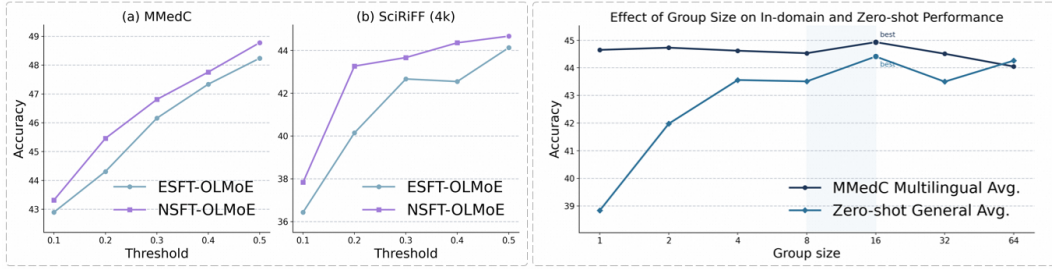
Figure 3: Threshold and group-size ablations. Left: performance under different selection thresholds on MMedC and SciRiFF. The NSFT results correspond to NSFT-SG, which uses learning-rate scaling and static gradient scaling. Right: effect of group size on in-domain (MMedC) and zero-shot general performance.
