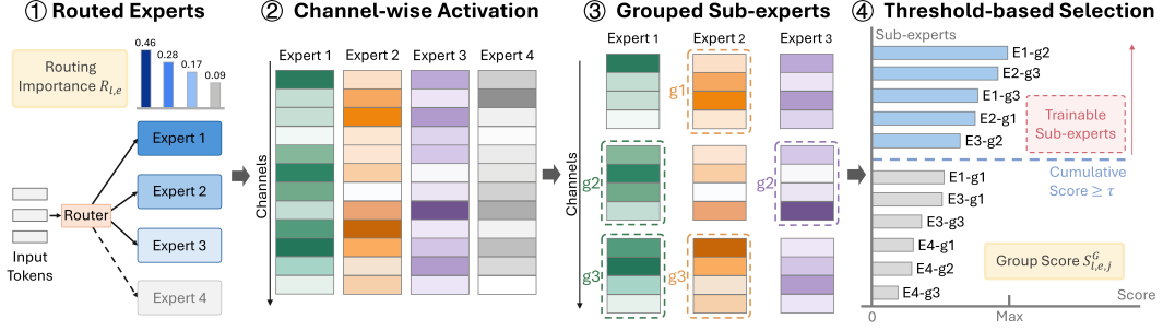
Figure 2: Illustration of sub-expert selection. Routed experts are first identified, and channel-wise activations are computed within each expert. With group size G = 4 , consecutive channels are partitioned into sub-expert groups, where E1-g1 denotes the first group of Expert 1. All groups are then scored and ranked, and the groups selected under the threshold \tau are used as trainable sub-experts for fine-tuning.
