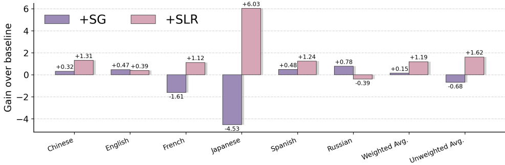
Figure 4: Ablation of gradient scaling (+SG) and learning-rate scaling (+SLR) on MMedC multilingual subtasks using OLMoE. Bars show gains over the NSFT baseline, i.e., the variant with only sub-expert selection and no adaptive training strategy.
