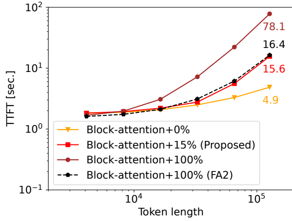
Figure 11: Averaged TTFT over 20 tasks in the RULER HQA using Llama3.1-8B-Instruct with the number of documents per cache file set to 16. TTFT of full attention with FlashAttention-2 (FA2) is comparable to that of 15% recomputation with Flashinfer.
