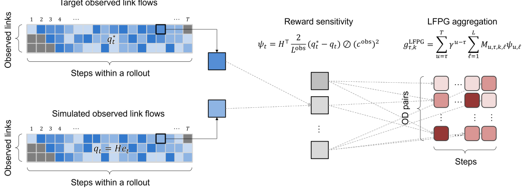
Figure 3: Construction of LFPG from propagated volumes and link-flow mismatch.
