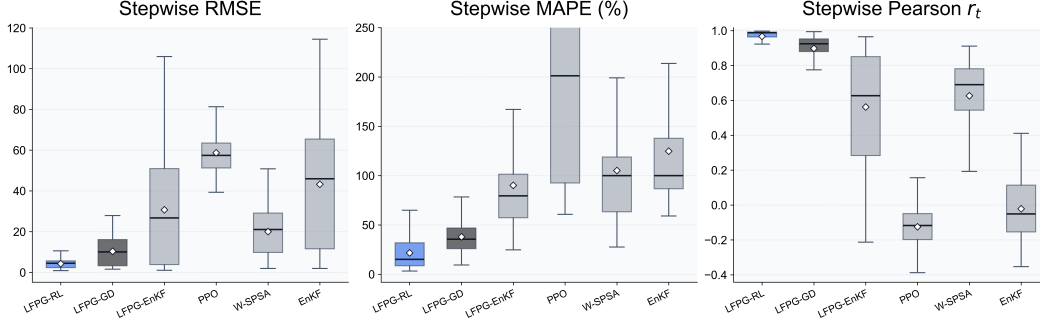
Figure 8: Distribution of stepwise RMSE, MAPE, and Pearson r_t across methods.
