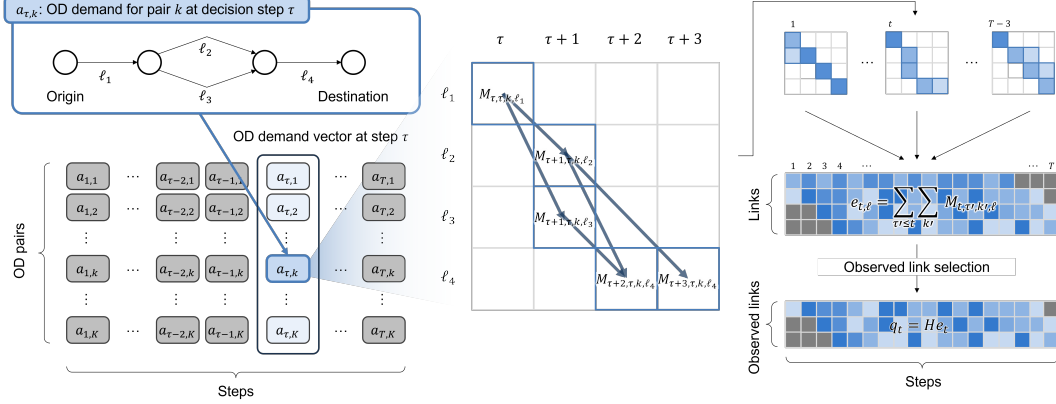
Figure 2: Extraction of link-flow propagation information from an OD-time demand component.
