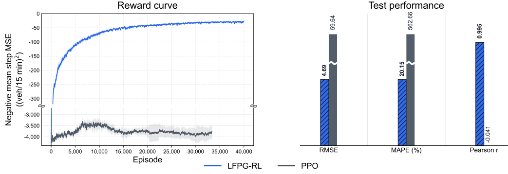
Figure 6: (a) Reward curve and (b) test performance comparison between LFPG-RL and PPO. Each policy was trained for 20 hours on a PC equipped with an AMD Threadripper PRO 5975WX.
