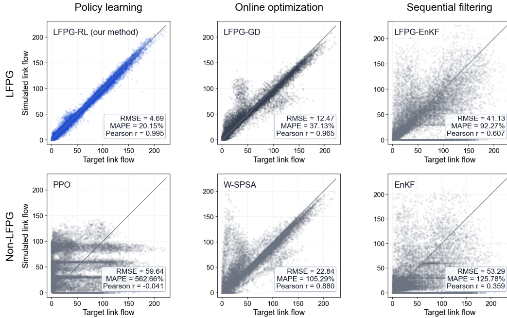
Figure 7: Target versus simulated link-flow scatter plots by methods.
