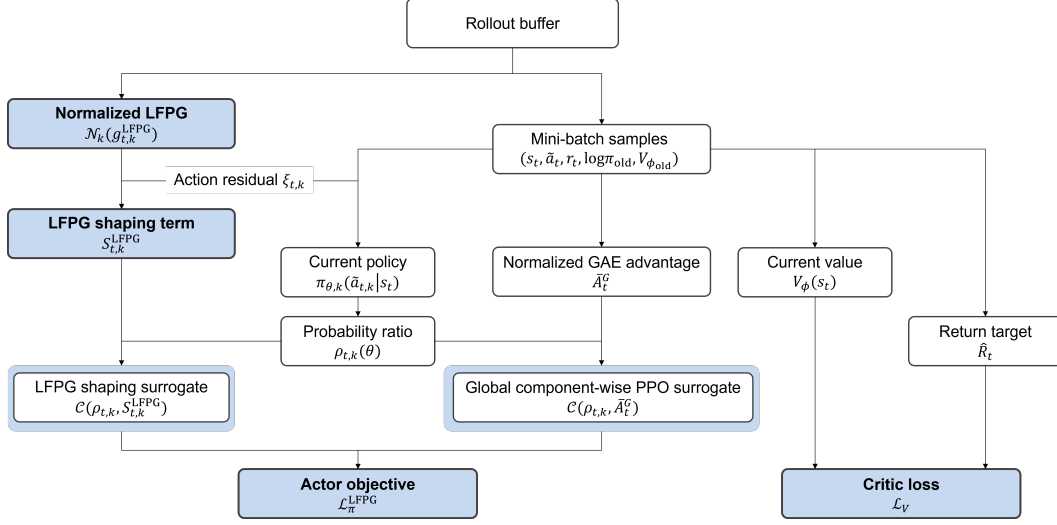
Figure 4: LFPG-RL policy update with global PPO advantage and OD-specific LFPG shaping.
