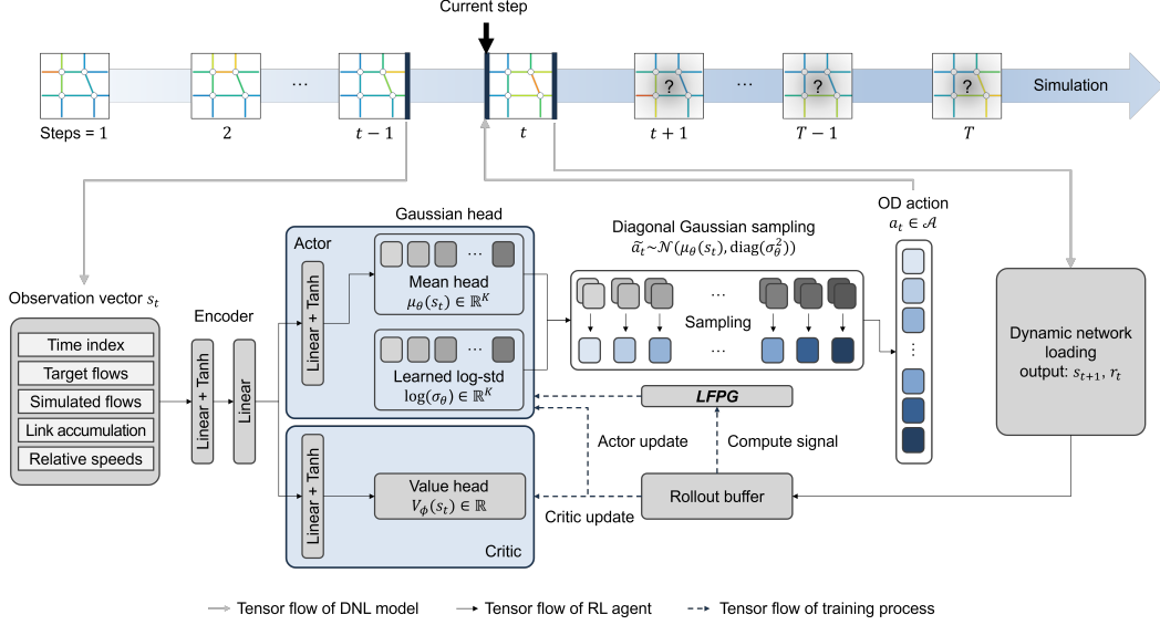
Figure 1: Overall framework of LFPG-RL for online DODE.
