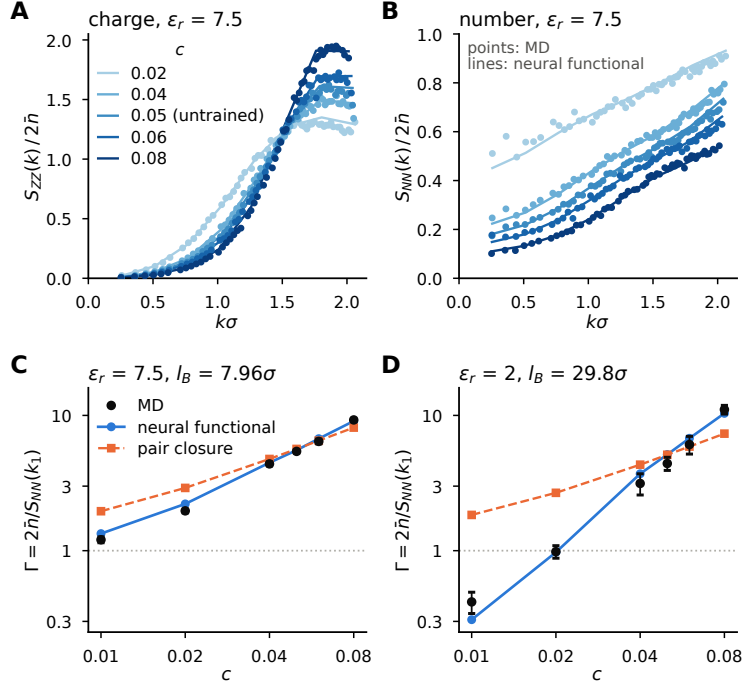
Figure 4. Bulk structure and long-wavelength number response. (A, B) Normalized charge and number structure factors at \epsilon_r = 7.5 and c = 0.02 to 0.08 . Points show zero-field MD results averaged over k -shells; curves show predictions from Eq. 7. (C, D) Finite-wavenumber response factor \Gamma(k_1) = 2\tilde{n}/S_{NN}(k_1) at \epsilon_r = 7.5 and 2 . Solid curves show the neural functional and dashed curves the pair closure. The dotted line marks the ideal value \Gamma = 1 . Neither quantity enters the force-matching loss.
