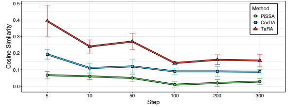
Figure 5: Gradient similarity, measured as the cosine similarity between the n -step (5, 10, 50, 100, 200 and 300) gradient of the combined LoRA adapter and that of the full weight, correlates with downstream accuracy.
