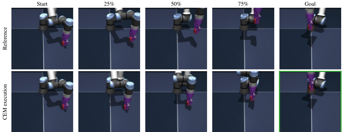
Fig. 2. Qualitative goal-conditioned planning on OGBench-Cube. Top: the reference trajectory between the fixed start and goal observations. Bottom: actual simulator observations obtained by executing CEM actions.
