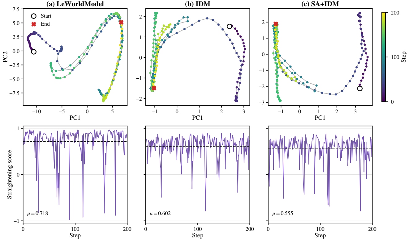
Fig. 3. Temporal straightening on a representative OGBench-Cube trajectory. Top: separate PCA projections of the encoded latent states, colored by time; circles and crosses mark the start and end. Bottom: local straightening scores, with dashed lines indicating trajectory means. All scores are computed in the full 192-dimensional latent space. The same qualitative pattern was observed across all sampled trajectories.
