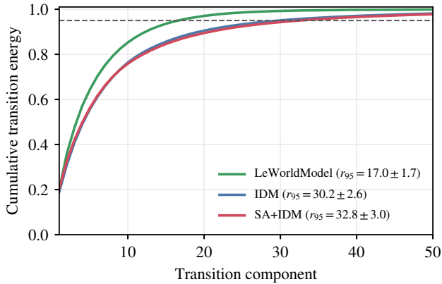
Fig. 4. Transition-subspace analysis over 100 fixed OGBench-Cube trajectories. Curves show mean cumulative transition energy under an uncentered SVD of \Delta z_t . Here, r_{95} is the number of components required to retain 95% of the energy.
