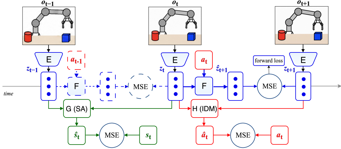
Fig. 1. Overview of the proposed model. The encoder E maps observations to latent representations, and the action-conditioned predictor F models their evolution. The inverse-dynamics head H predicts the executed action from consecutive representations, while the state-alignment head G grounds them in measured physical states. The dashed branch denotes the corresponding prediction at the preceding time step.
