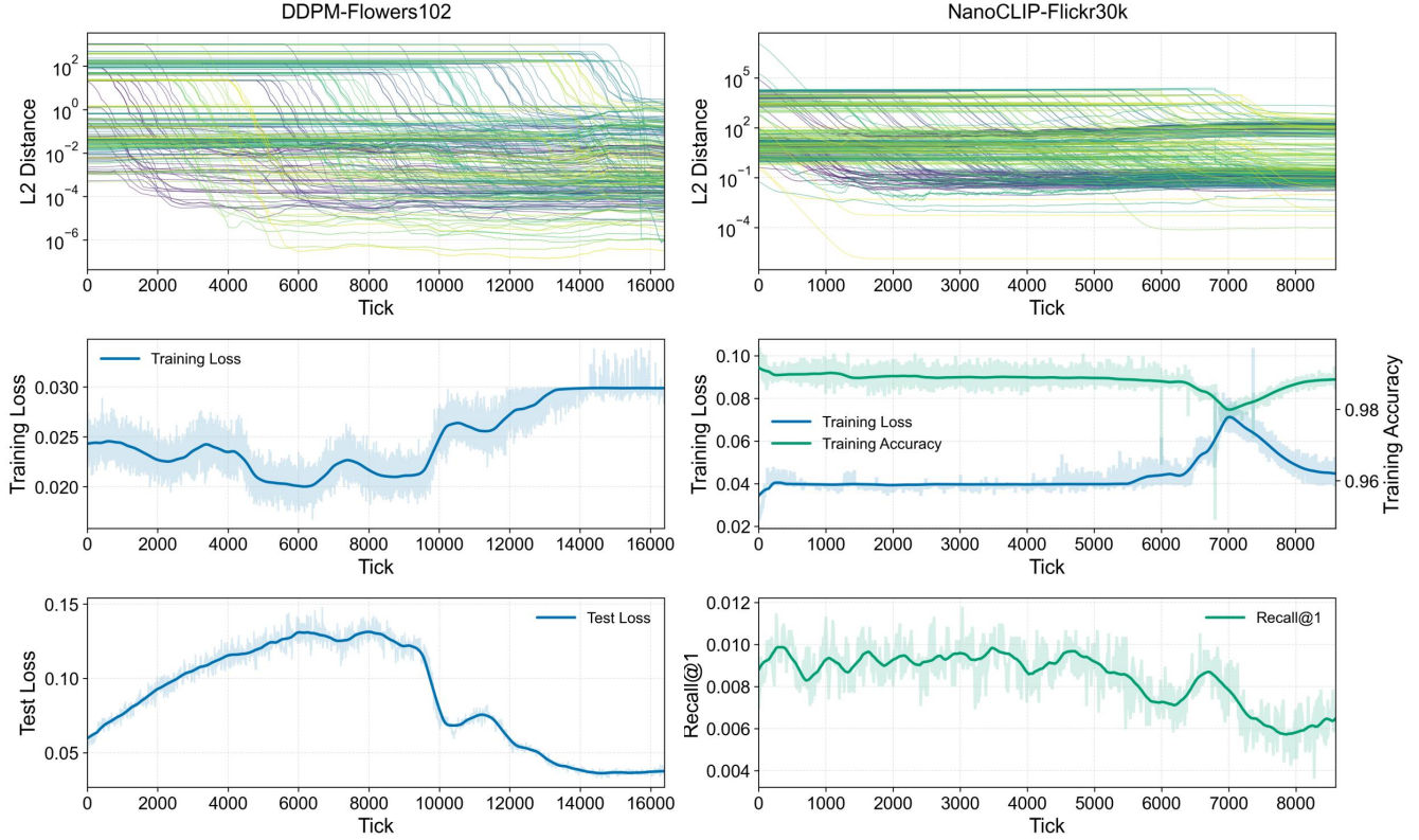
Figure 3: Results of the architecture-aware connection building algorithm on DDPM (first column) and NanoCLIP (second column). The first row shows the layer-wise L_2 distance from the current point P_i to the end mode P_E , and the legend of layers is omitted due to excessive quantity. The second and third rows respectively report the training and test metrics along the path. The curves show the smoothed trends, and the shaded regions indicate local fluctuation envelopes of the raw metrics. Due to the learning objectives of the models, DDPM is evaluated only with training and test losses, whereas NanoCLIP is evaluated without a test loss.
