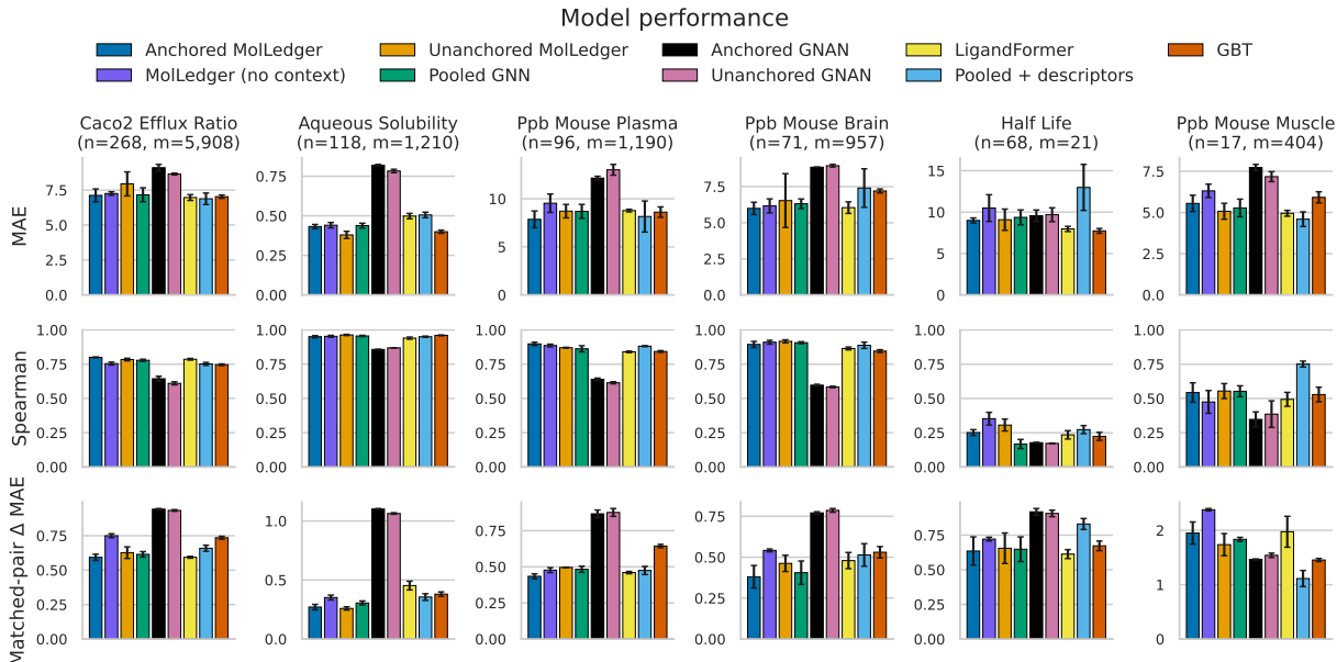
Figure 8: Performance on smaller tasks as a continuation of Figure 1. n is the number of test samples, and m is the number of matched pairs with a molecule from the test set. Mean and standard deviation across 3 random seeds.
