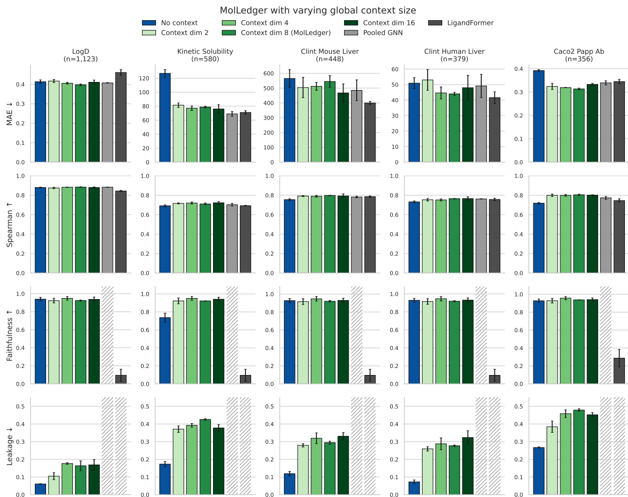
Figure 4: Performance of MolLedger when varying global context vector dimension. The no-context MolLedger uses the sum and mean form in Figure 5. All variants of MolLedger are trained with the anchor loss. Faithfulness and leakage are not measured for the pooled GNN as they depend on the interpretability method applied. Leakage is not defined for LigandFormer.
