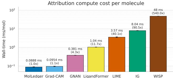
Figure 7: Time to run each interpretability method.
