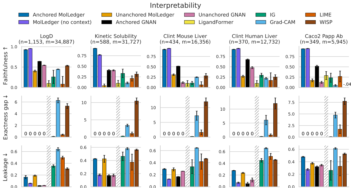
Figure 2: Interpretability metrics evaluated on the held-out test set for the 5 largest tasks. n is the number of test samples, and m is the number of matched pairs with a molecule from the test set. Mean and standard deviation across 3 random seeds. Methods were not penalized for their bias terms when computing the exactness gap, and changes in the core atom attached to the substituent are not penalized in leakage. Exactness gap and leakage are not defined for LigandFormer’s attention scores. Remaining tasks are shown in Figure 9 in Appendix D.
