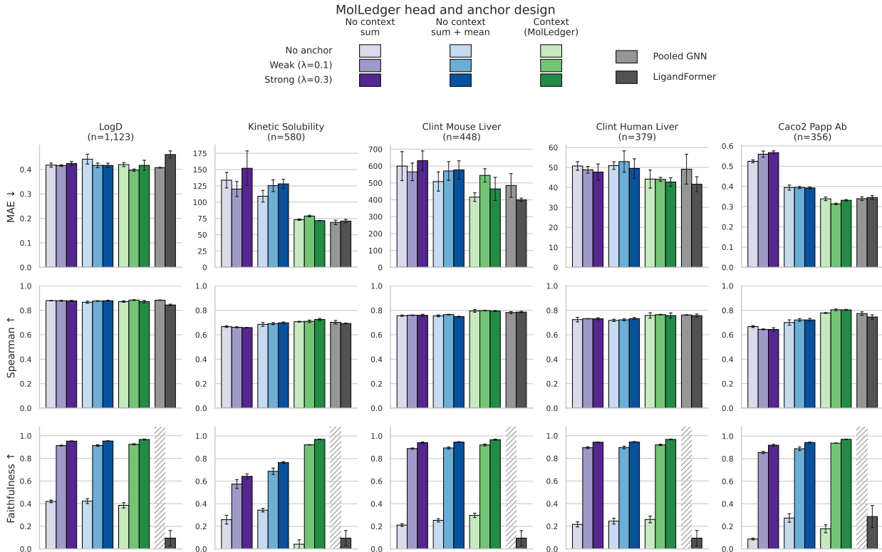
Figure 5: Performance of MolLedger with varying anchor strength. Three types of heads are evaluated for MolLedger. Faithfulness is not measured for the pooled GNN as it depends on the interpretability method applied.
