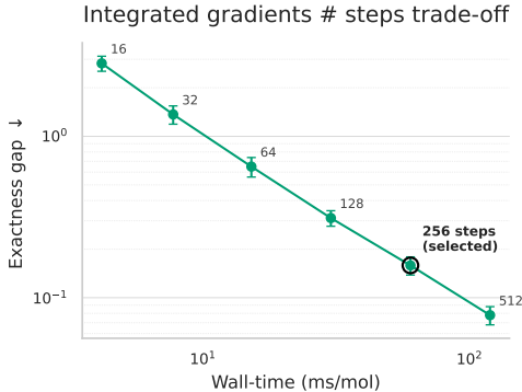
Figure 6: Exactness vs time trade-off for integrated gradients.
