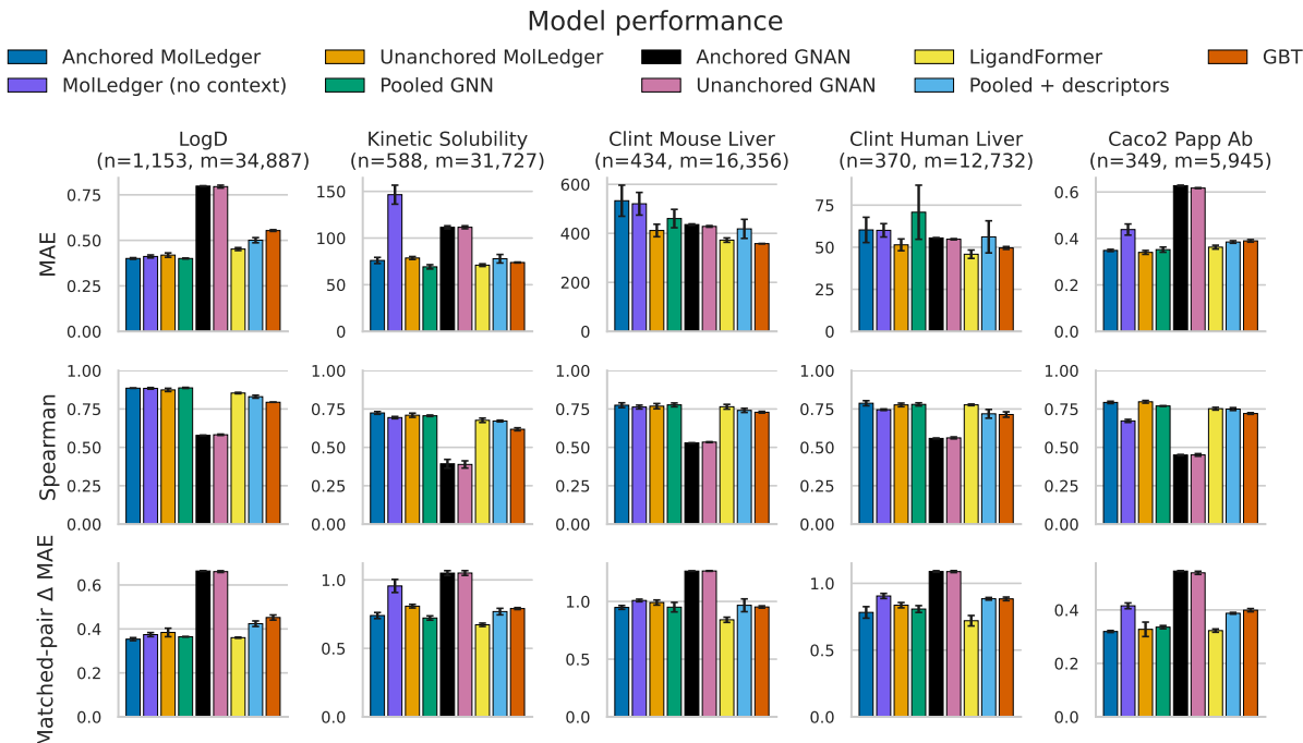
Figure 1: Performance on the held-out test set for the 5 largest tasks. n is the number of test samples, and m is the number of matched pairs with a molecule from the test set. Mean and standard deviation across 3 random seeds. Remaining tasks are shown in Figure 8 in Appendix D.
