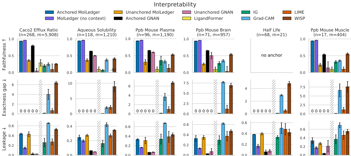
Figure 9: Interpretability metrics on smaller tasks as a continuation of Figure 2. n is the number of test samples, and m is the number of matched pairs with a molecule from the test set. Mean and standard deviation across 3 random seeds. Exactness gap and leakage are not defined for LigandFormer's attention scores.
