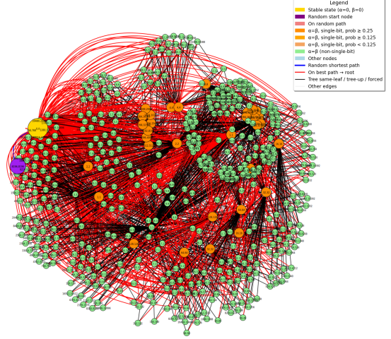
(b) DT guided graph of SIMECK32
