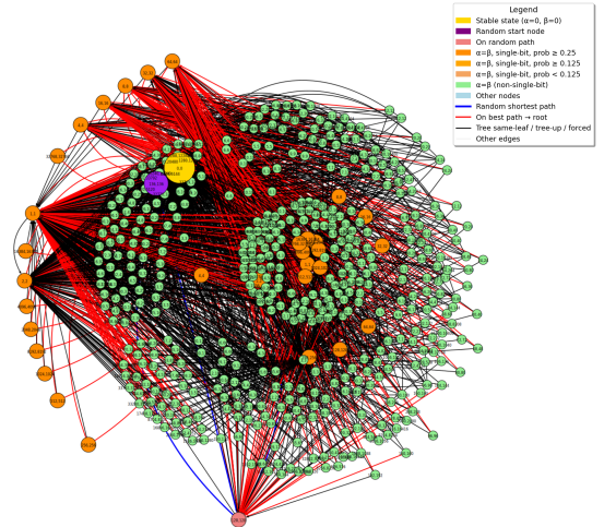
(b) RF guided graph of SIMECK32
