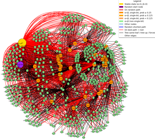
(a) DT guided graph of SIMON32
