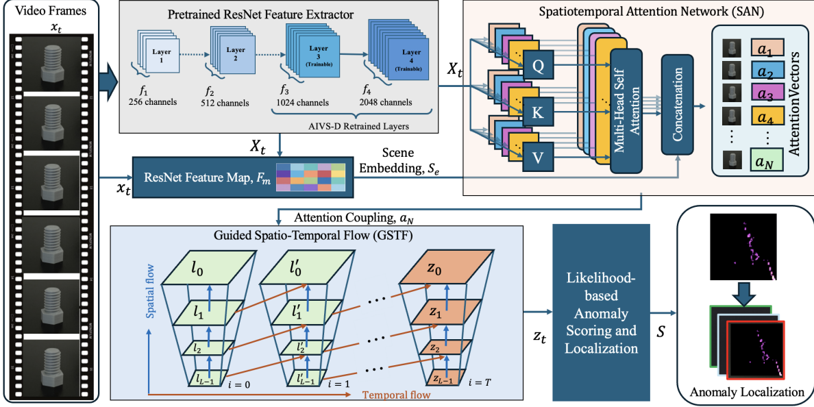
Figure 1. GuidedFlow Overview. The model is composed of four parts: ResNet Feature Extractor, Spatio-temporal Attention Network, Guided Spatio-Temporal Flow, and Anomaly Localization Map.
