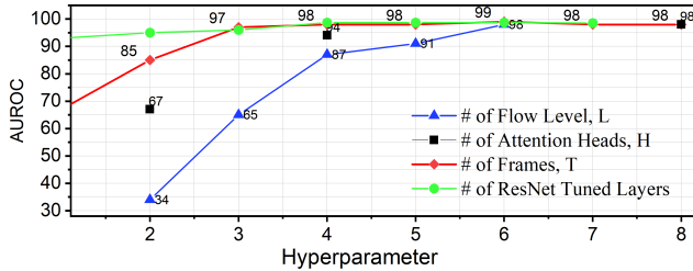
Figure 4. GuidedFlow hyperparameter performance. AUROC values for the hyperparameter settings are shown as percentages (%).
