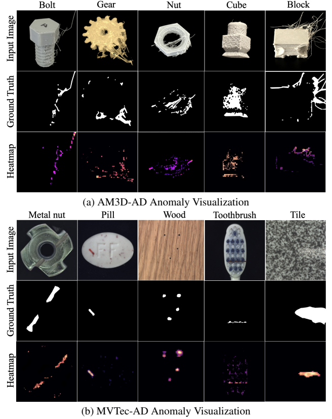
Figure 3. Visualization of GuidedFlow anomaly localization results on AM3D-AD and MVTec-AD datasets. The top row is input images, the middle row ground truths, and the bottom row GuidedFlow localization as heatmaps, where higher intensity values indicate a higher anomaly likelihood
