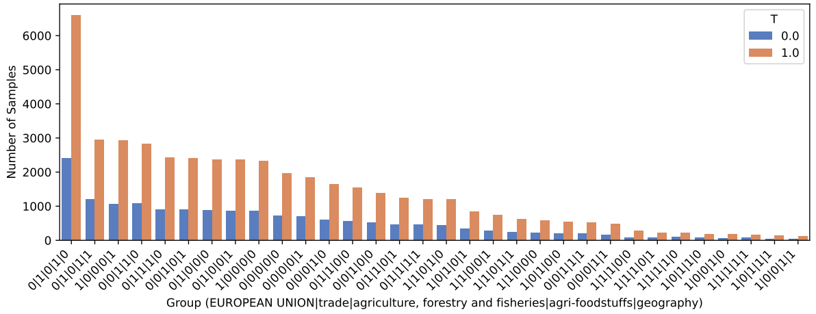
Figure 11: Treatment assignment on EURLEX
