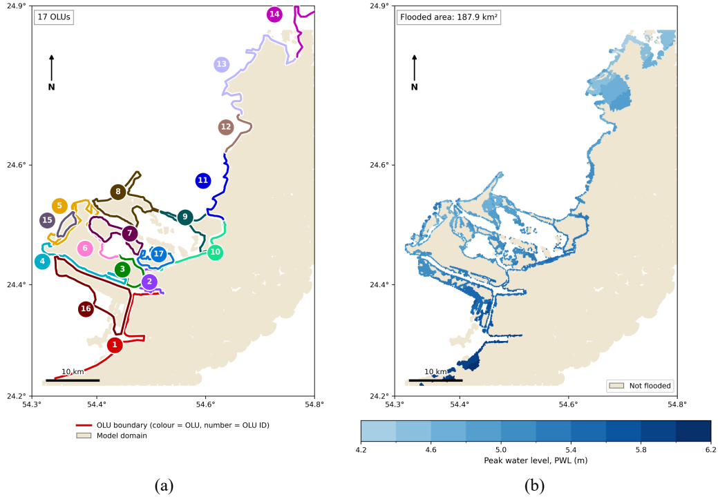
Figure 5: Abu Dhabi study region. (a) The 17 OLUs, with each shoreline segment colored and numbered by its OLU. (b) Simulated PWL at 0.5 m SLR when no OLU is protected, giving a flooded area of 187.9 km 2 .
