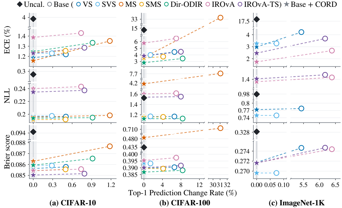
Figure 2: Post-fit prediction preservation. ECE, NLL, and Brier versus TPCR on CIFAR-10/100 and ImageNet-1K. Dashed lines pair each direct output with its CORD repair, and the gray band marks TPCR = 0. Markers are dataset-wise averages over classifiers and five splits.
