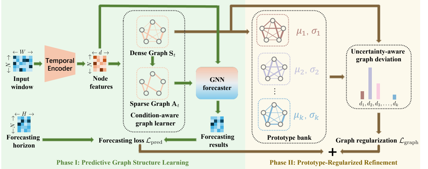
Figure 1: Overview of GSLAD. In Phase I, the temporal encoder, condition-aware graph learner, and GNN forecaster are optimized using predictive supervision. Dense normal graphs are clustered into multiple uncertainty-aware prototypes, while sparsified graphs are used for efficient GNN processing. In Phase II, deviation from the prototype bank regularizes graph learning. During inference, uncertainty-aware structural deviation and predictive deviation are combined for anomaly scoring.
