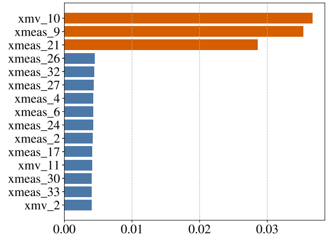
Figure 4: Node-level deviation ranking.
