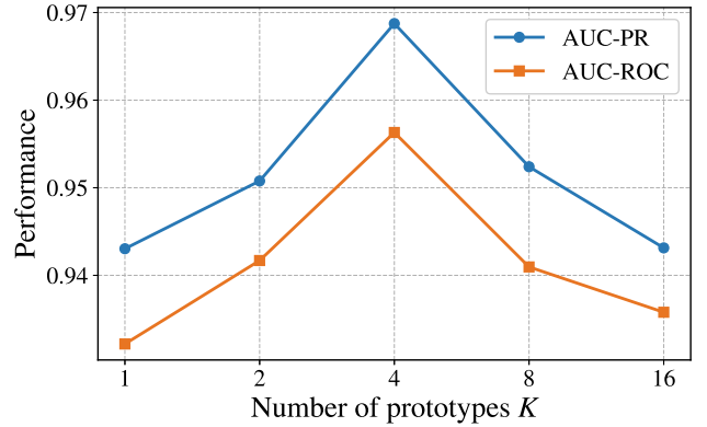
Figure 2: Sensitivity to prototype number K .
