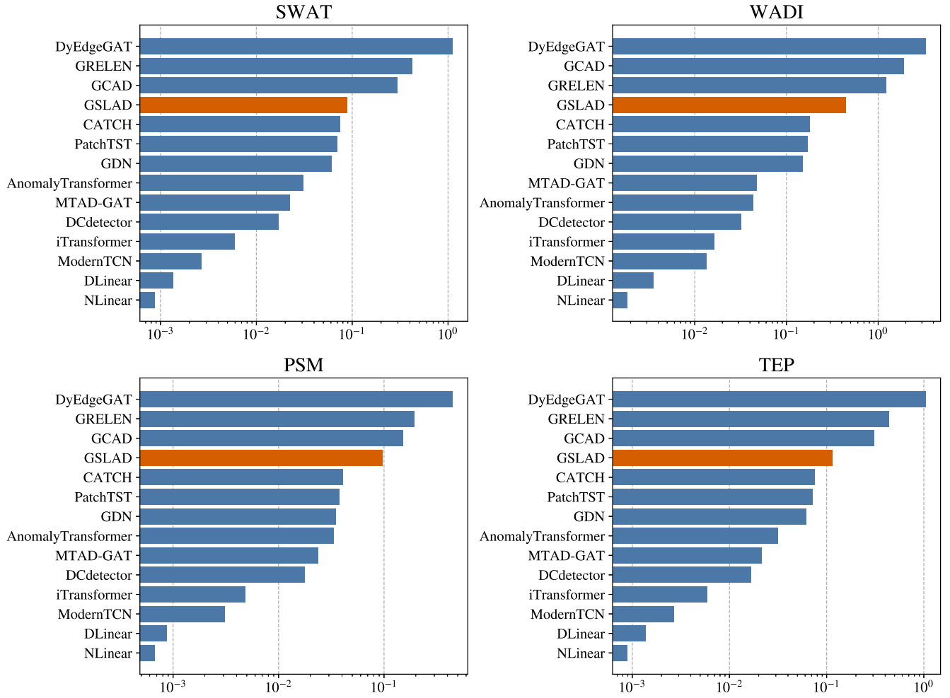
Figure 5: Per-sample inference time comparison.
