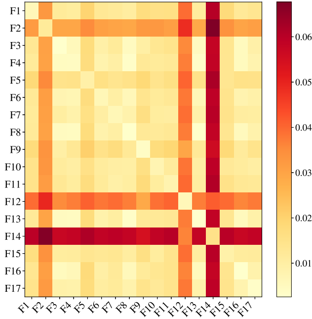
Figure 3: Cross-fault structural matrix.
