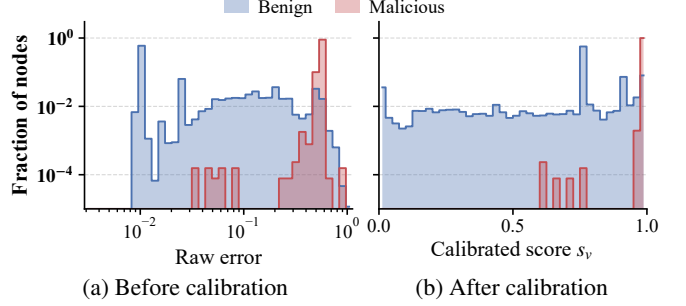
Fig. 3. Score distributions of benign and malicious nodes before and after relation-conditional calibration on CADETS.
