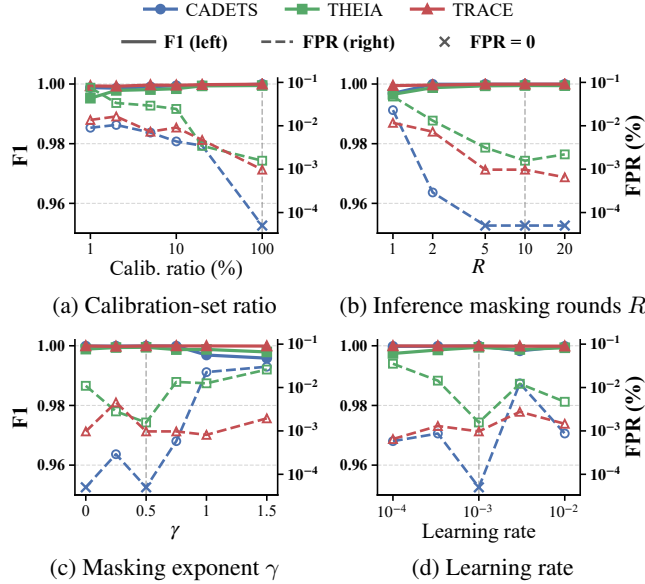
Fig. 4. Parameter sensitivity of RECAL. Solid lines show F1 (left axis) and dashed lines show FPR (right axis, log scale).
