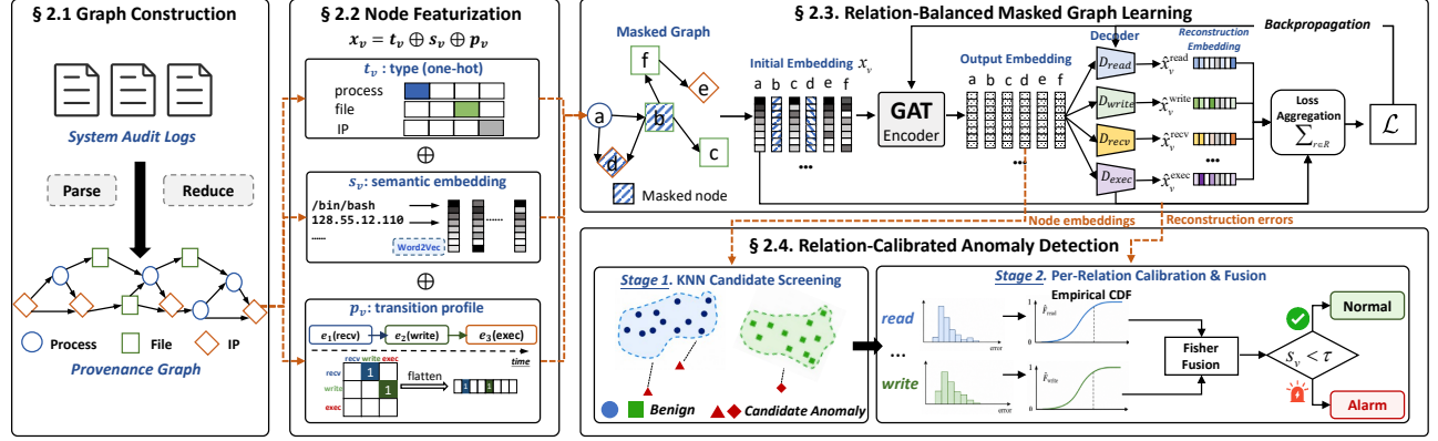
Fig. 2. Overview of RECAL. Graph construction and node featurization transform audit logs into attributed provenance graphs for relation-balanced masked graph learning. Node embeddings support KNN candidate screening, while relation-specific reconstruction errors support candidate calibration and evidence fusion for final detection. Orange dashed arrows indicate data flow between modules.
