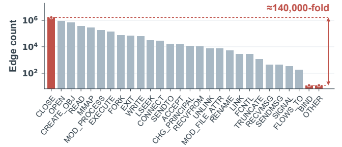
Fig. 1. CADETS benign training graphs. The x-axis shows audit-log relations; the y-axis shows event counts (log scale).
