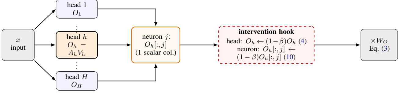
Figure 2. Where the interventions sit inside one attention layer. Every head’s output O_h (Eq. (2)) is an additive term (Eq. (3)); ablating head h zeroes its whole term, while ablating neuron j zeroes only one column of O_h . The forward-pre-hook on W_O ’s input (HeadSuppressor / NeuronSuppressor) implements both.
