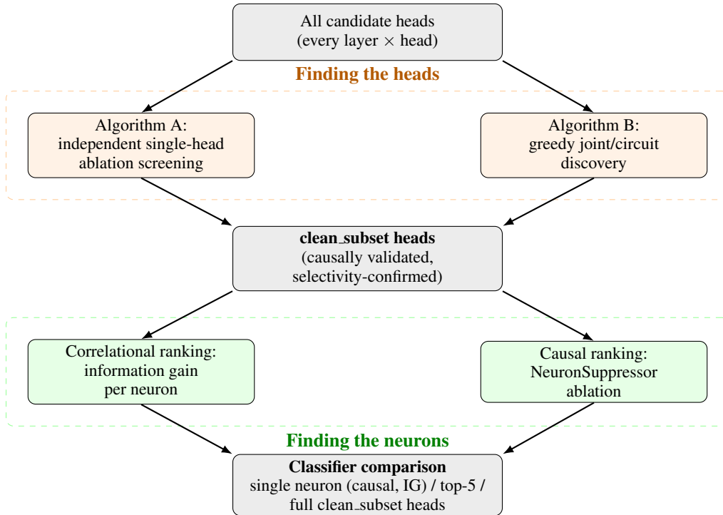
Figure 1. Pipeline overview. Two independent algorithms discover candidate heads and are cross-validated against each other; the surviving clean_subset heads then feed a second, structurally identical cross-validation at neuron granularity (correlational information-gain ranking vs. causal ablation), whose agreement or disagreement is this paper’s central result (Section 4.2).
