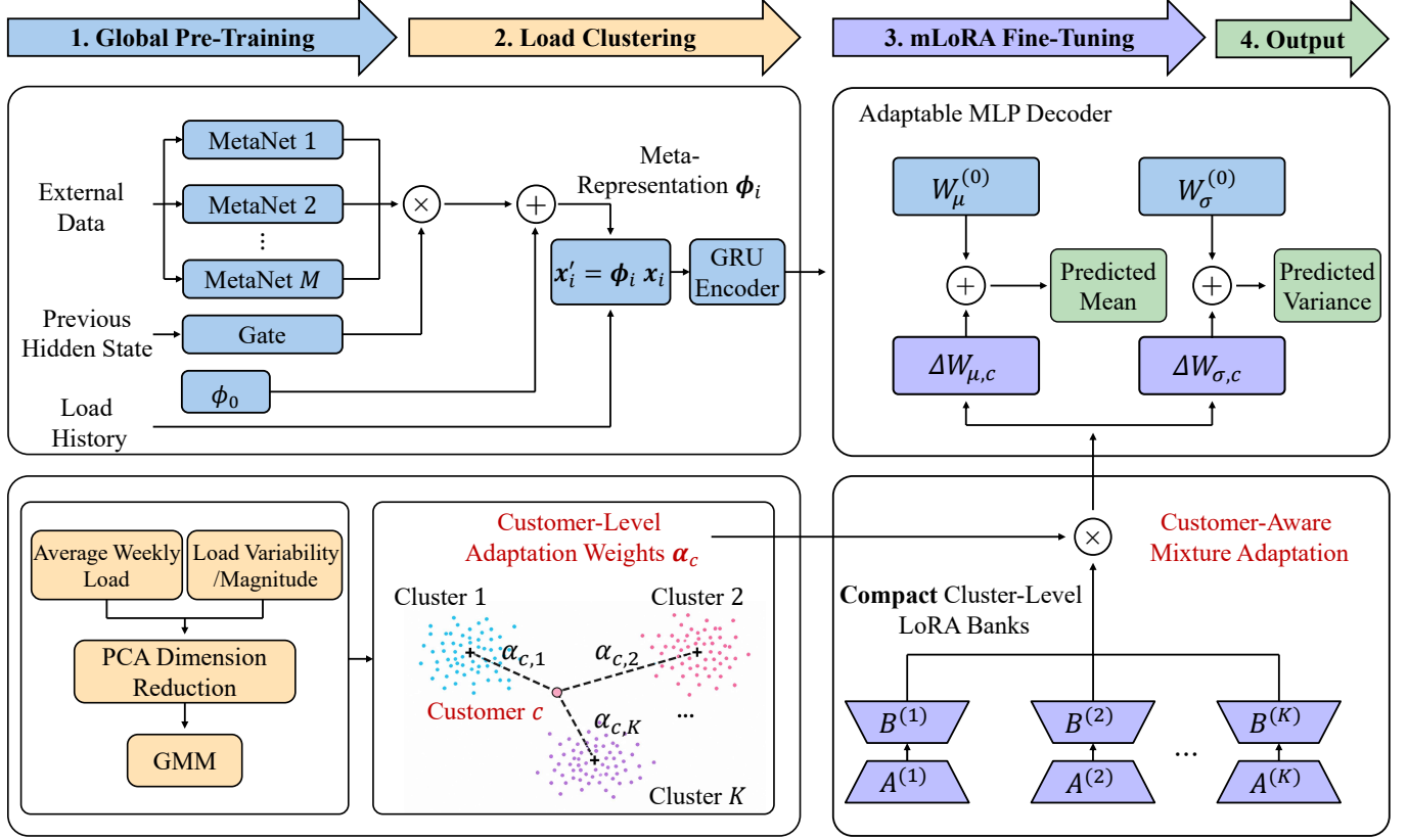
Fig. 1: M²oE²-mLoRA framework.
