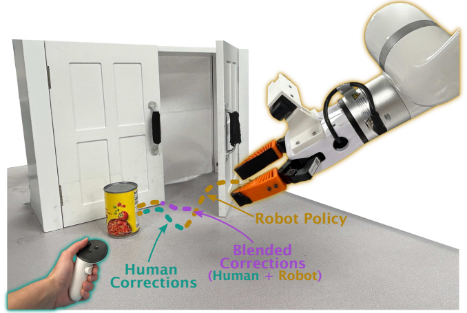
Fig. 1: BlenDagger shares control between the robot’s policy and the human demonstrator during corrections, resulting in higher autonomous success and faster data collection.
