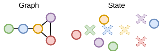
Figure 2: Example of a GRAFO task with five agents (circles). Left: agent graph identifying the task. Right: current state of the environment, where the green solid cross is the landmark known to all agents, i.e., the target position of the green agent, while the dashed crosses are the target positions of other agents. These positions are defined based on the graph, but are not explicitly provided.
