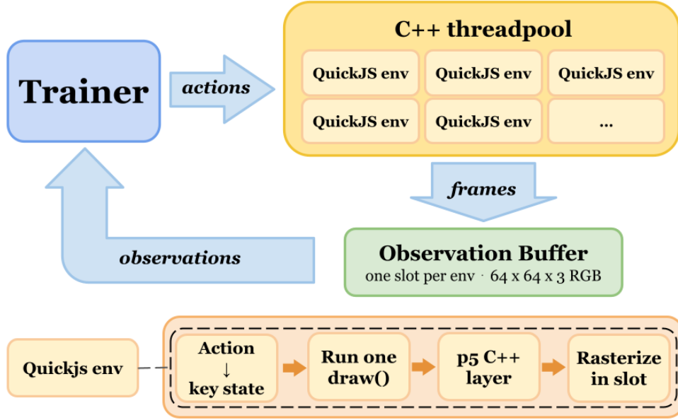
Figure 3: PlayTrain training schematic. A trainer sends actions to multiple environment instances hosted in an in-process C++ threadpool. Each instance is an embedded QuickJS engine running the game file behind our optimized C++ p5 library and custom Rust rasterizer. Each instance writes its frames directly into its own slot of the shared observation buffer ( 64 \times 64 \times 3 RGB), which the trainer reads as observations. In each instance: per step, the environment receives an action and transforms it into a keyboard state and then runs a single draw() . Our C++ p5 API intercepts those draw calls, and our rasterizer executes them at observation resolution directly into that environment’s slot.
