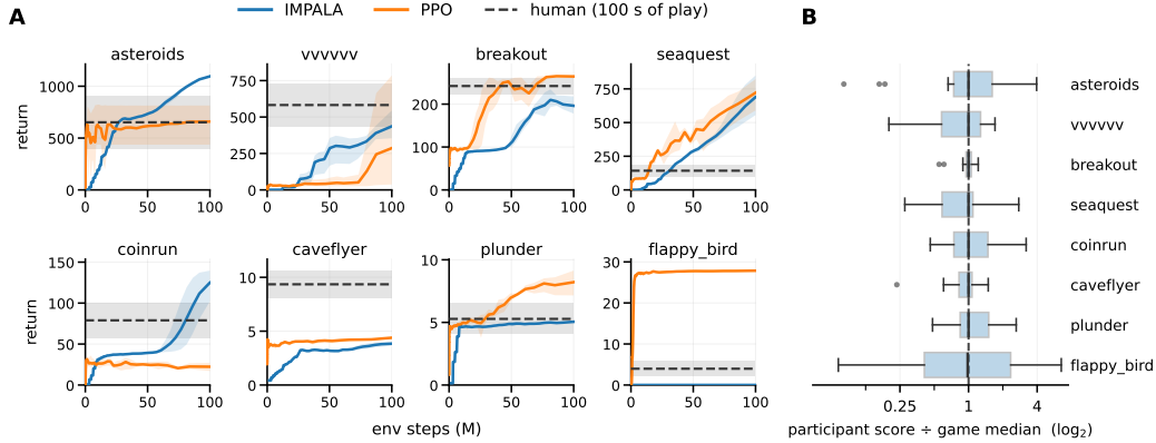
Figure 6: (A) Comparing IMPALA and PPO agent training efficiency against 100 seconds of human play. Dashed horizontal lines are the human mean over 20 participants and the gray band is the 95% confidence interval. Solid curves are the RL agents’ means over three seeds, shaded with min–max bands. Both RL agents use the IMPALA-CNN encoder. (B) The distribution of the 20 participants’ scores on each game. Each participant’s score is divided by that game’s median so that all the games can share the same axis.
