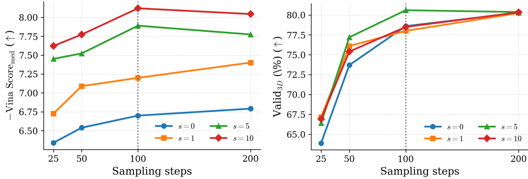
Figure 5: Sampling-step ablation under representative CFG scales. Left: median Vina Score is shown as -Vina Score_{med} , so higher is better. Right: Valid_{3D} under the GenBench3D protocol. The vertical dashed line marks the default setting N = 100 .
