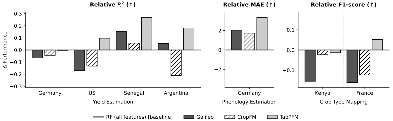
Figure 2: Relative Performance Gap. The zero-line represents the unconstrained Random Forest baseline utilizing all available dataset specific modalities. Bars show the relative performance ( \Delta ) of models restricted to their natively supported modalities and evaluated using frozen features and a Random Forest. To ensure positive values always indicate improvement, \Delta is computed as Model – Baseline for R^2 and F1-score, and Baseline – Model for MAE. Negative values explicitly highlight the performance gap incurred from missing dataset-critical modalities.
