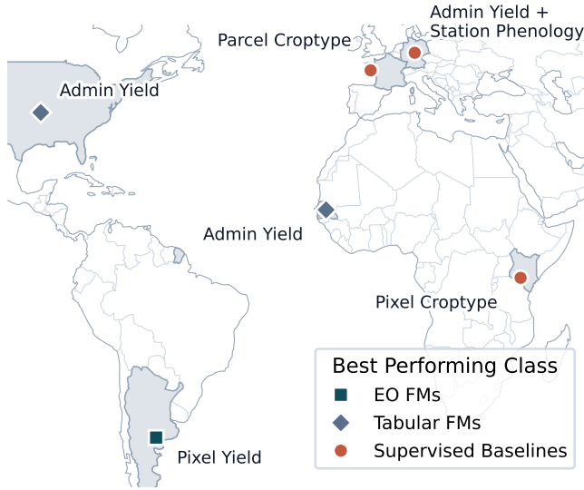
Figure 1: The map (left) demonstrates the geographic diversity of our evaluation and highlights the winning model family for each region. The absence of a universal winner is driven by the structural complexity of the tasks, which vary drastically across five key dimensions of shifts (right).
