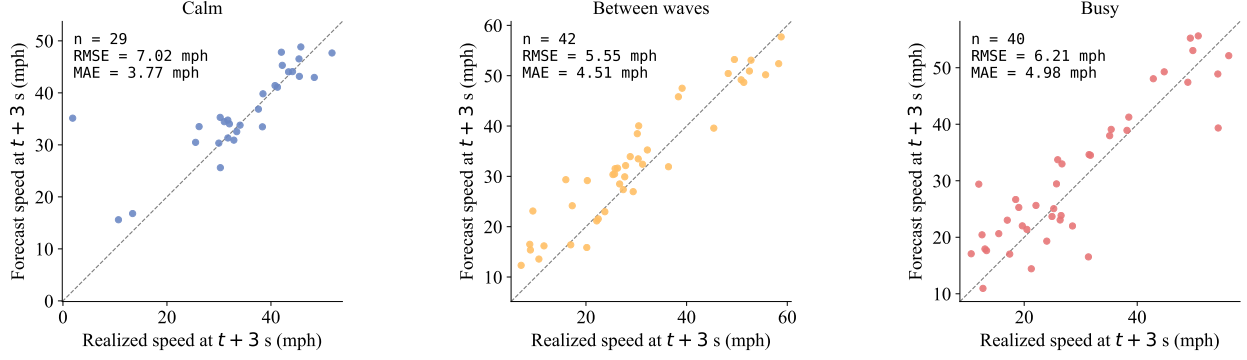
Figure 21: Short-horizon (3s) forecast of human-driver speed from the trained state representation, evaluated on lane 1 of I-24 MOTION under calm, busy, and between-waves conditions. Each point is one vehicle; axes compare forecast and realized speed at the 3s horizon, with the diagonal marking perfect prediction.
