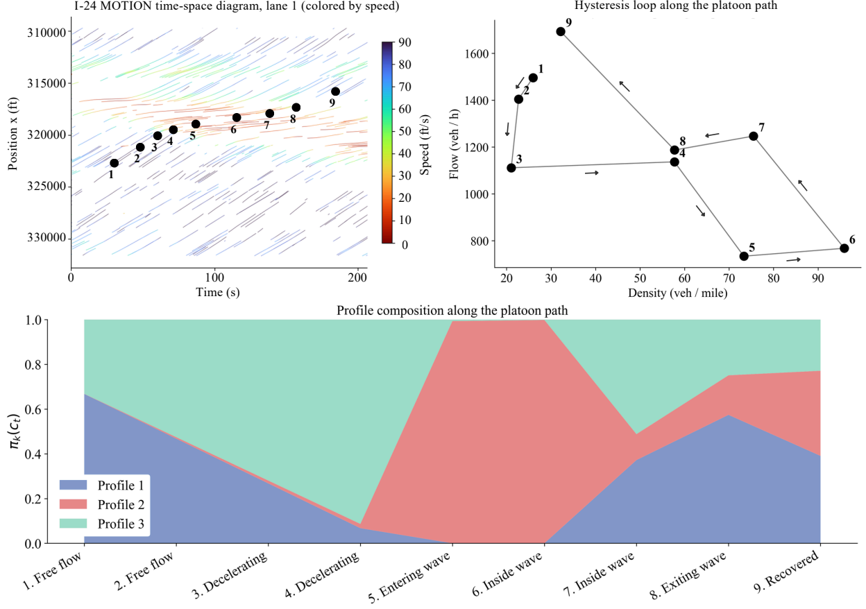
Figure 18: Hysteresis on a westbound I-24 MOTION wave (lane 1). Top left : the wave on the time-space diagram. Top right : the resulting ( density , flow ) traced through a representative trajectory. Bottom : the average profile composition \pi_k(c_t) at each point.
