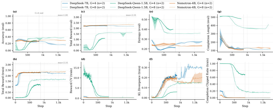
Figure 3: GRPO training dynamics on OpenCoder across models and group sizes ( G \in \{4, 8\} ). Performance and reward improve rapidly before reaching diminishing returns, while larger G provides only model-dependent gains. KL remains bounded, entropy generally decreases, and completion lengths vary substantially across models.
