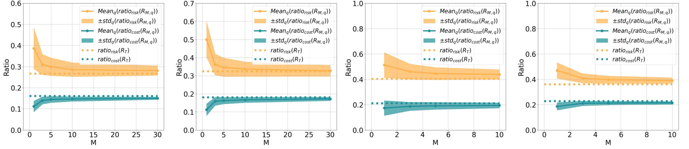
(a) Audit cost ratio ( \text{ratio}_{\text{cost}} ) versus audit risk ratio ( \text{ratio}_{\text{risk}} ) as a function of the size of the retail ensemble. Results are shown (Left to Right) for: BERT on SST2 , RoBERTa on MRPC , BIG-SCIENCE T0 on Bank , BIG-SCIENCE T0 on Adult . Increasing the ensemble size has a small impact in matching the warehouse once the ensemble is sufficiently large (around M=10 ).
