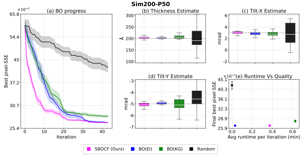
Figure H12: Results for Sim200-P50 with ground-truth thickness 200 Å, tilts (3, -5) mrad, and Poisson noise with a peak photon count of 50. Panels show (a) best observed pixel-wise SSE, final estimates of (b) thickness, (c) tilt-X, and (d) tilt-Y, and (e) acquisition runtime versus final SSE. Solid lines in Panel (a) show the mean across 20 trials, and the shaded regions indicate standard error. Dashed lines in Panels (b)–(d) indicate the ground truth.
