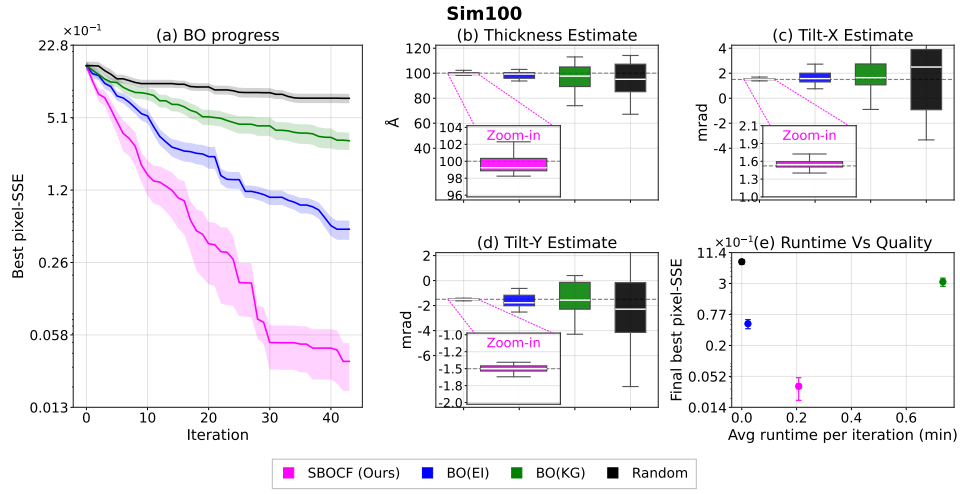
Figure F1: Results for Sim100 with ground-truth thickness 100 \text{ \AA} and tilts (1.5, -1.5) \text{ mrad} . Layout and conventions as in Fig. 4.
