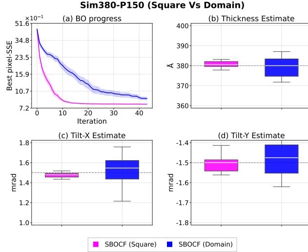
Figure I3: Comparison of SBOCF using the square and domain partition patterns on the Sim380-P150 problem with ground-truth thickness 380 Å, tilts (1.5, −1.5) mrad and Poisson noise with a peak photon count of 150. Panels show (a) best observed pixel-wise SSE and final estimates of (b) thickness, (c) tilt-X, and (d) tilt-Y. Solid lines in Panel (a) show the mean across 20 trials, and the shaded regions indicate standard error. Dashed lines in Panels (b)–(d) indicate the ground truth.
