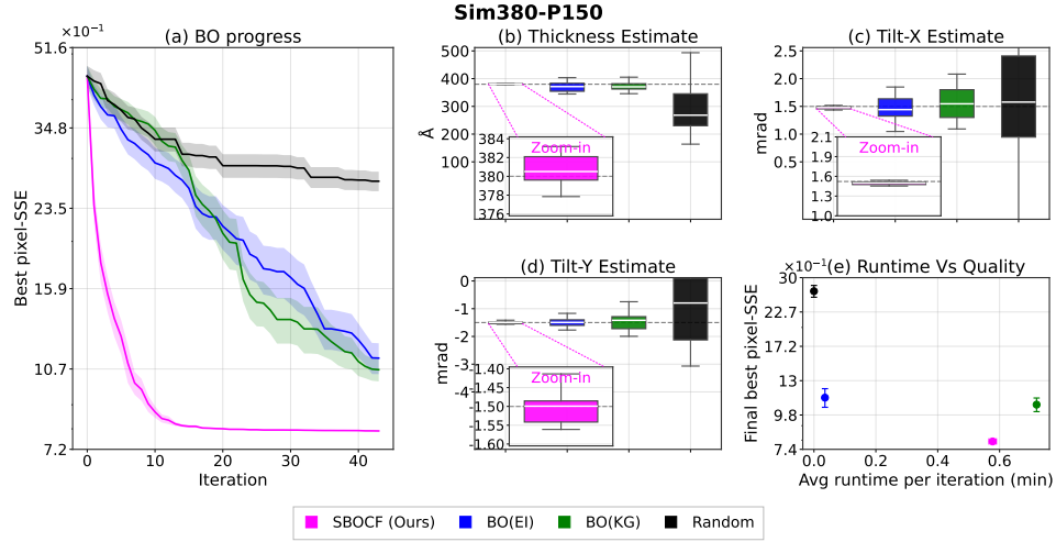
Figure H4: Results for Sim380-P150 with ground-truth thickness 380 Å, tilts (1.5, -1.5) mrad, and Poisson noise with a peak photon count of 150. Panels show (a) best observed pixel-wise SSE, final estimates of (b) thickness, (c) tilt-X, and (d) tilt-Y, and (e) acquisition runtime versus final SSE. Solid lines in Panel (a) show the mean across 20 trials, and the shaded regions indicate standard error. Dashed lines in Panels (b)–(d) indicate the ground truth.
