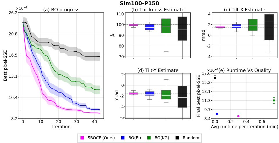
Figure H7: Results for Sim100-P150 with ground-truth thickness 100 \text{ \AA} , tilts (1.5, -1.5) \text{ mrad} , and Poisson noise with a peak photon count of 150. Panels show (a) best observed pixel-wise SSE, final estimates of (b) thickness, (c) tilt-X, and (d) tilt-Y, and (e) acquisition runtime versus final SSE. Solid lines in Panel (a) show the mean across 20 trials, and the shaded regions indicate standard error. Dashed lines in Panels (b)–(d) indicate the ground truth.
