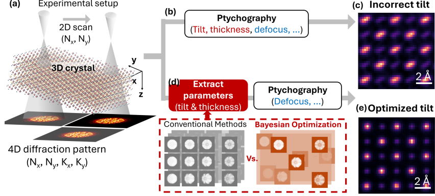
Figure 1: Conceptual workflow for PACBED-based specimen-parameter estimation prior to MEP. (a) A 4D-STEM dataset is acquired from a specimen with unknown thickness and mistilt. (b) Conventionally these parameters are estimated jointly with the other reconstruction variables, and (c) uncorrected mistilt degrades the result. (d) In the proposed workflow they are estimated first, by comparing the experimental PACBED pattern with multislice simulations: conventional methods evaluate a predefined grid, whereas BO-based methods adaptively select candidates from previous results. (e) The improved reconstruction expected after correction.
