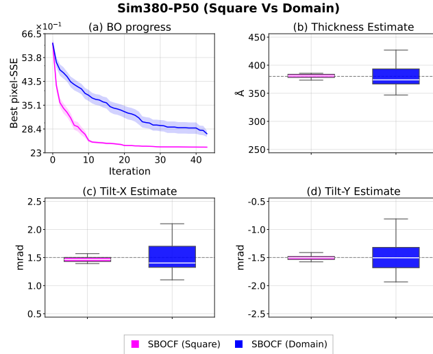
Figure I5: Comparison of SBOCF using the square and domain partition patterns on the Sim380-P50 problem with ground-truth thickness 380 Å, tilts (1.5, -1.5) mrad and Poisson noise with a peak photon count of 50. Panels show (a) best observed pixel-wise SSE and final estimates of (b) thickness, (c) tilt-X, and (d) tilt-Y. Solid lines in Panel (a) show the mean across 20 trials, and the shaded regions indicate standard error. Dashed lines in Panels (b)–(d) indicate the ground truth.
