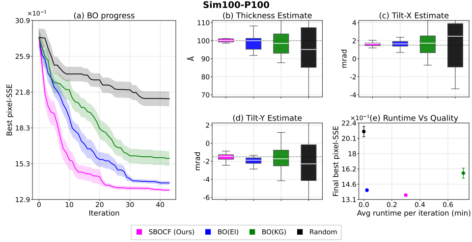
Figure H8: Results for Sim100-P100 with ground-truth thickness 100 Å, tilts (1.5, -1.5) mrad, and Poisson noise with a peak photon count of 100. Panels show (a) best observed pixel-wise SSE, final estimates of (b) thickness, (c) tilt-X, and (d) tilt-Y, and (e) acquisition runtime versus final SSE. Solid lines in Panel (a) show the mean across 20 trials, and the shaded regions indicate standard error. Dashed lines in Panels (b)–(d) indicate the ground truth.
