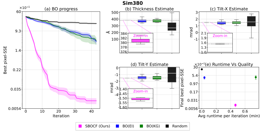
Figure 4: Results for Sim380 with ground-truth thickness 380 \text{ \AA} and tilts (1.5, -1.5) \text{ mrad} . Panels show (a) best observed pixel-wise SSE, final estimates of (b) thickness, (c) tilt-X, and (d) tilt-Y, and (e) acquisition runtime versus final SSE. Solid lines in Panel (a) show the mean across 20 trials, and the shaded regions indicate standard error. Dashed lines in Panels (b)–(d) indicate the ground truth.
