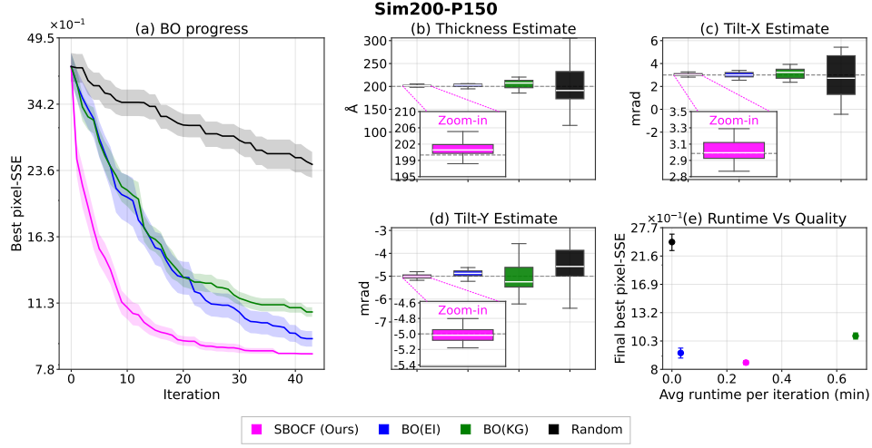
Figure H10: Results for Sim200-P150 with ground-truth thickness 200 \text{ \AA} , tilts (3, -5) \text{ mrad} , and Poisson noise with a peak photon count of 150. Panels show (a) best observed pixel-wise SSE, final estimates of (b) thickness, (c) tilt-X, and (d) tilt-Y, and (e) acquisition runtime versus final SSE. Solid lines in Panel (a) show the mean across 20 trials, and the shaded regions indicate standard error. Dashed lines in Panels (b)–(d) indicate the ground truth.
