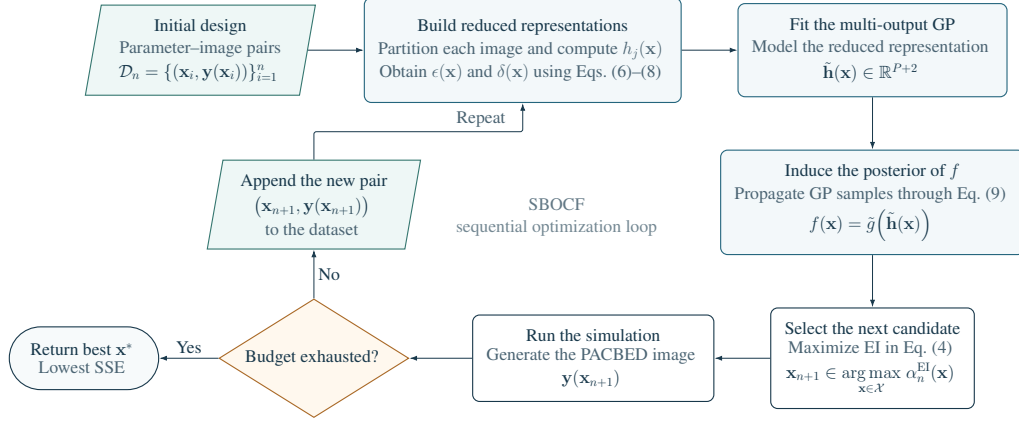
Figure 3: Flowchart of the proposed SBOCF algorithm.
