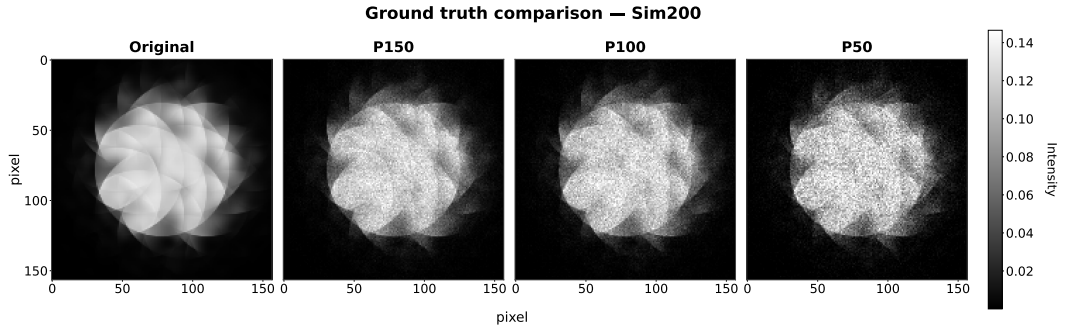
Figure H3: Comparison between the original ground truth PACBED pattern and noisy observations for the Sim200 benchmark problem with a sample thickness of 200 Å. From left to right, the figure shows the original noise-free image and noisy versions generated using peak photon counts of P150, P100, and P50. Lower peak photon counts correspond to higher levels of Poisson noise.
