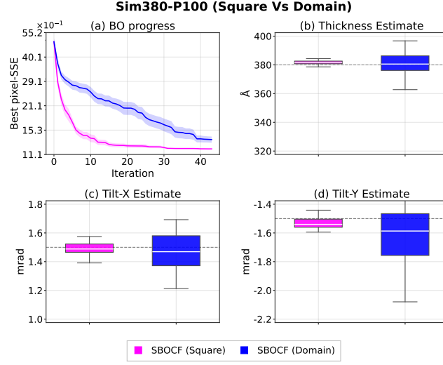
Figure I4: Comparison of SBOCF using the square and domain partition patterns on the Sim380-P100 problem with ground-truth thickness 380 Å, tilts (1.5, -1.5) mrad and Poisson noise with a peak photon count of 100. Panels show (a) best observed pixel-wise SSE and final estimates of (b) thickness, (c) tilt-X, and (d) tilt-Y. Solid lines in Panel (a) show the mean across 20 trials, and the shaded regions indicate standard error. Dashed lines in Panels (b)–(d) indicate the ground truth.
