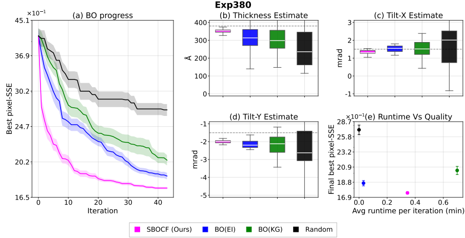
Figure 5: Results for the Exp380 experimental \text{SrTiO}_3 PACBED benchmark using the target image from [6]. Layout as in Fig. 4, except that dashed lines in Panels (b)–(d) indicate the reference estimates reported in [6].
