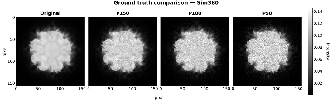
Figure H1: Comparison between the original ground truth PACBED pattern and noisy observations for the Sim380 benchmark problem with a sample thickness of 380 Å. From left to right, the figure shows the original noise-free image and noisy versions generated using peak photon counts of P150, P100, and P50. Lower peak photon counts correspond to higher levels of Poisson noise.
