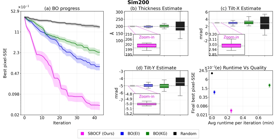
Figure G1: Results for Sim200 with ground-truth thickness 200 Å and tilts (3, -5) mrad. Layout and conventions as in Fig. 4.
