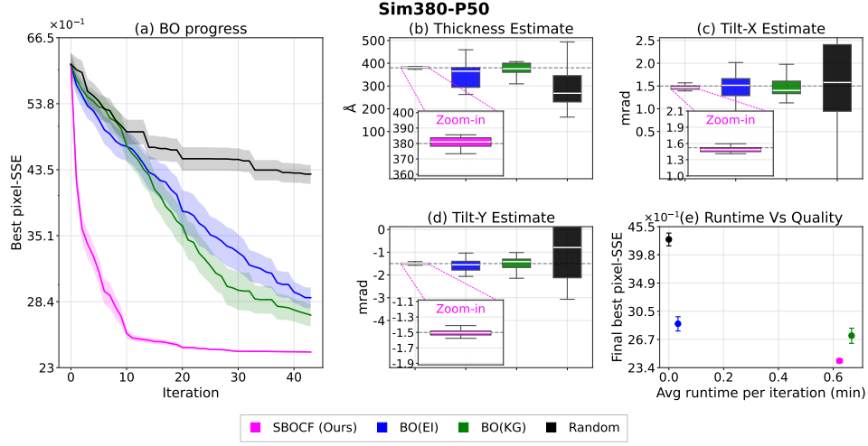
Figure H6: Results for Sim380-P50 with ground-truth thickness 380 \text{ \AA} , tilts (1.5, -1.5) \text{ mrad} , and Poisson noise with a peak photon count of 50. Panels show (a) best observed pixel-wise SSE, final estimates of (b) thickness, (c) tilt-X, and (d) tilt-Y, and (e) acquisition runtime versus final SSE. Solid lines in Panel (a) show the mean across 20 trials, and the shaded regions indicate standard error. Dashed lines in Panels (b)–(d) indicate the ground truth.
