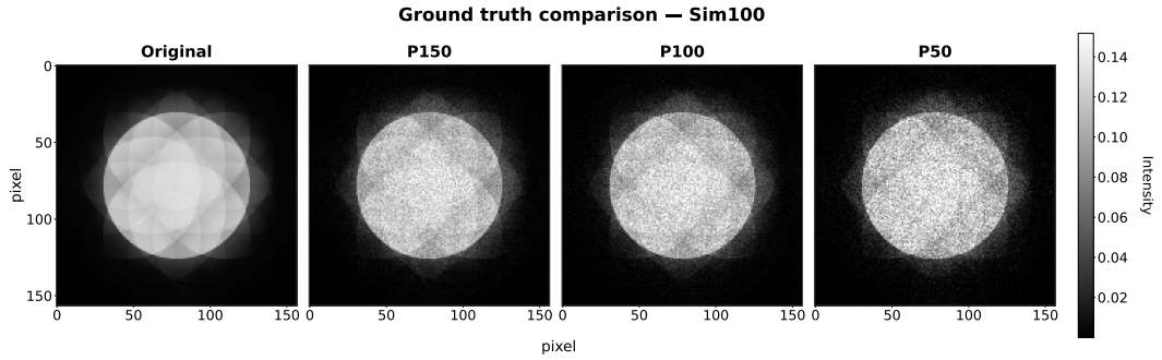
Figure H2: Comparison between the original ground truth PACBED pattern and noisy observations for the Sim100 benchmark problem with a sample thickness of 100 Å. From left to right, the figure shows the original noise-free image and noisy versions generated using peak photon counts of P150, P100, and P50. Lower peak photon counts correspond to higher levels of Poisson noise.
