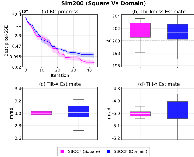
Figure I10: Comparison of SBOCF using the square and domain partition patterns on the noiseless Sim200 problem with ground-truth thickness 200 \text{ \AA} and tilts (3, -5) \text{ mrad} . Panels show (a) best observed pixel-wise SSE and final estimates of (b) thickness, (c) tilt-X, and (d) tilt-Y. Solid lines in Panel (a) show the mean across 20 trials, and the shaded regions indicate standard error. Dashed lines in Panels (b)–(d) indicate the ground truth.
