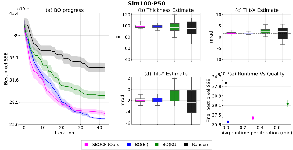
Figure H9: Results for Sim100-P50 with ground-truth thickness 100 Å, tilts (1.5, -1.5) mrad, and Poisson noise with a peak photon count of 50. Panels show (a) best observed pixel-wise SSE, final estimates of (b) thickness, (c) tilt-X, and (d) tilt-Y, and (e) acquisition runtime versus final SSE. Solid lines in Panel (a) show the mean across 20 trials, and the shaded regions indicate standard error. Dashed lines in Panels (b)–(d) indicate the ground truth.
