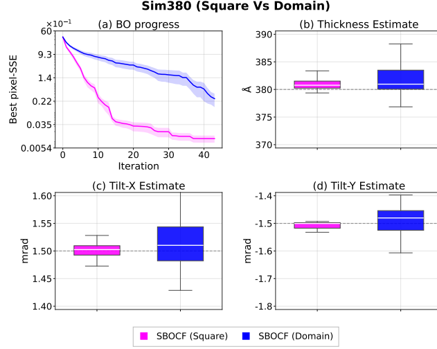
Figure I2: Comparison of SBOCF using the square and domain partition patterns on the noiseless Sim380 problem with ground-truth thickness 380 Å and tilts (1.5, −1.5) mrad. Panels show (a) best observed pixel-wise SSE and final estimates of (b) thickness, (c) tilt-X, and (d) tilt-Y. Solid lines in Panel (a) show the mean across 20 trials, and the shaded regions indicate standard error. Dashed lines in Panels (b)–(d) indicate the ground truth.
