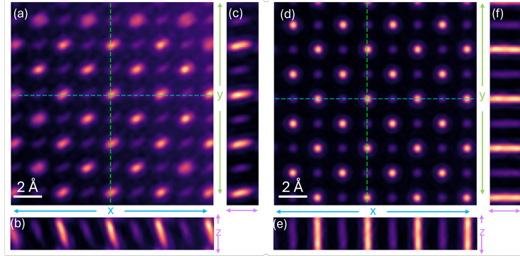
Figure 6: Effect of specimen mistilt on multislice electron ptychography and its correction using SBOCF estimates, for a simulated \text{SrTiO}_3 specimen of thickness 200 Å with tilts of 3 mrad (tilt-X) and −5 mrad (tilt-Y). (a)–(c) Reconstruction of the dataset without accounting for the tilt: (a) projected view, (b) x – z and (c) y – z depth sections. (d)–(f) The corresponding reconstruction using the SBOCF-estimated parameters
