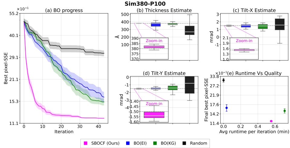
Figure H5: Results for Sim380-P100 with ground-truth thickness 380 Å, tilts (1.5, -1.5) mrad, and Poisson noise with a peak photon count of 100. Panels show (a) best observed pixel-wise SSE, final estimates of (b) thickness, (c) tilt-X, and (d) tilt-Y, and (e) acquisition runtime versus final SSE. Solid lines in Panel (a) show the mean across 20 trials, and the shaded regions indicate standard error. Dashed lines in Panels (b)–(d) indicate the ground truth.
