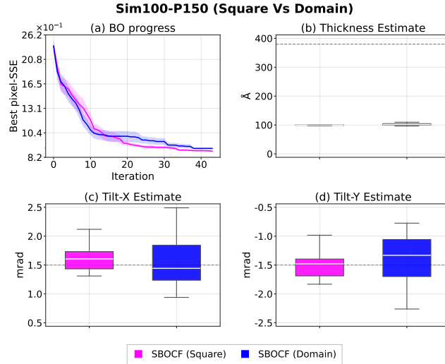
Figure I7: Comparison of SBOCF using the square and domain partition patterns on the Sim100-P150 problem with ground-truth thickness 100 \text{ \AA} , tilts (1.5, -1.5) \text{ mrad} and Poisson noise with a peak photon count of 150. Panels show (a) best observed pixel-wise SSE and final estimates of (b) thickness, (c) tilt-X, and (d) tilt-Y. Solid lines in Panel (a) show the mean across 20 trials, and the shaded regions indicate standard error. Dashed lines in Panels (b)–(d) indicate the ground truth.
