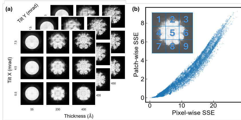
Figure 2: (a) PACBED patterns simulated for SrTiO 3 across thickness (columns) and tilt along two orthogonal axes, tiltX (rows) and tiltY (offset diagonally). Thickness reorganizes the fringe structure non-monotonically, while tilt along either axis breaks the pattern's symmetry in a direction-dependent way. (b) Pixel-wise SSE f(\mathbf{x}) versus patch-level SSE f^P(\mathbf{x}) for simulated PACBED images; their systematic relationship motivates using the patch-level SSE with correction terms.
