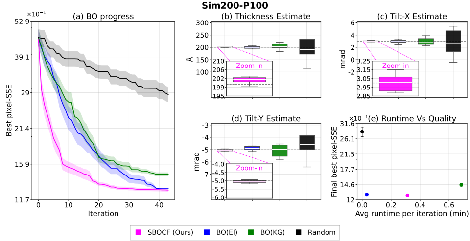
Figure H11: Results for Sim200-P100 with ground-truth thickness 200 \text{ \AA} , tilts (3, -5) \text{ mrad} , and Poisson noise with a peak photon count of 100. Panels show (a) best observed pixel-wise SSE, final estimates of (b) thickness, (c) tilt-X, and (d) tilt-Y, and (e) acquisition runtime versus final SSE. Solid lines in Panel (a) show the mean across 20 trials, and the shaded regions indicate standard error. Dashed lines in Panels (b)–(d) indicate the ground truth.
