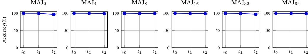
Figure 2: Length generalization accuracy of \mathcal{T} on MAJ k tasks.
