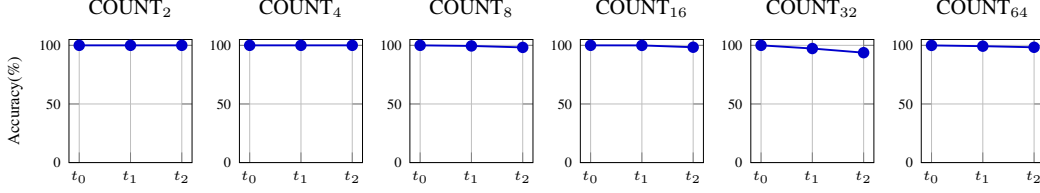
Figure 1: Length generalization accuracy of \mathcal{T} on COUNT k tasks.
