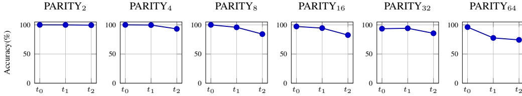
Figure 3: Length generalization accuracy of \mathcal{T} on PARITY k tasks.
