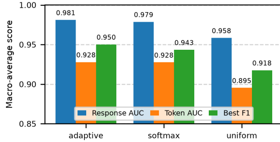
Figure 4: The ablation study of the token weighting techniques.
