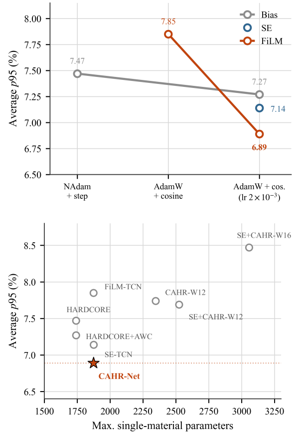
Fig. 6. Injection-optimization interaction and parameter efficiency. (a) Interaction between condition injection strategy and optimization protocol. (b) Parameter-count and average- p_{95} Pareto distribution of internal model variants.
