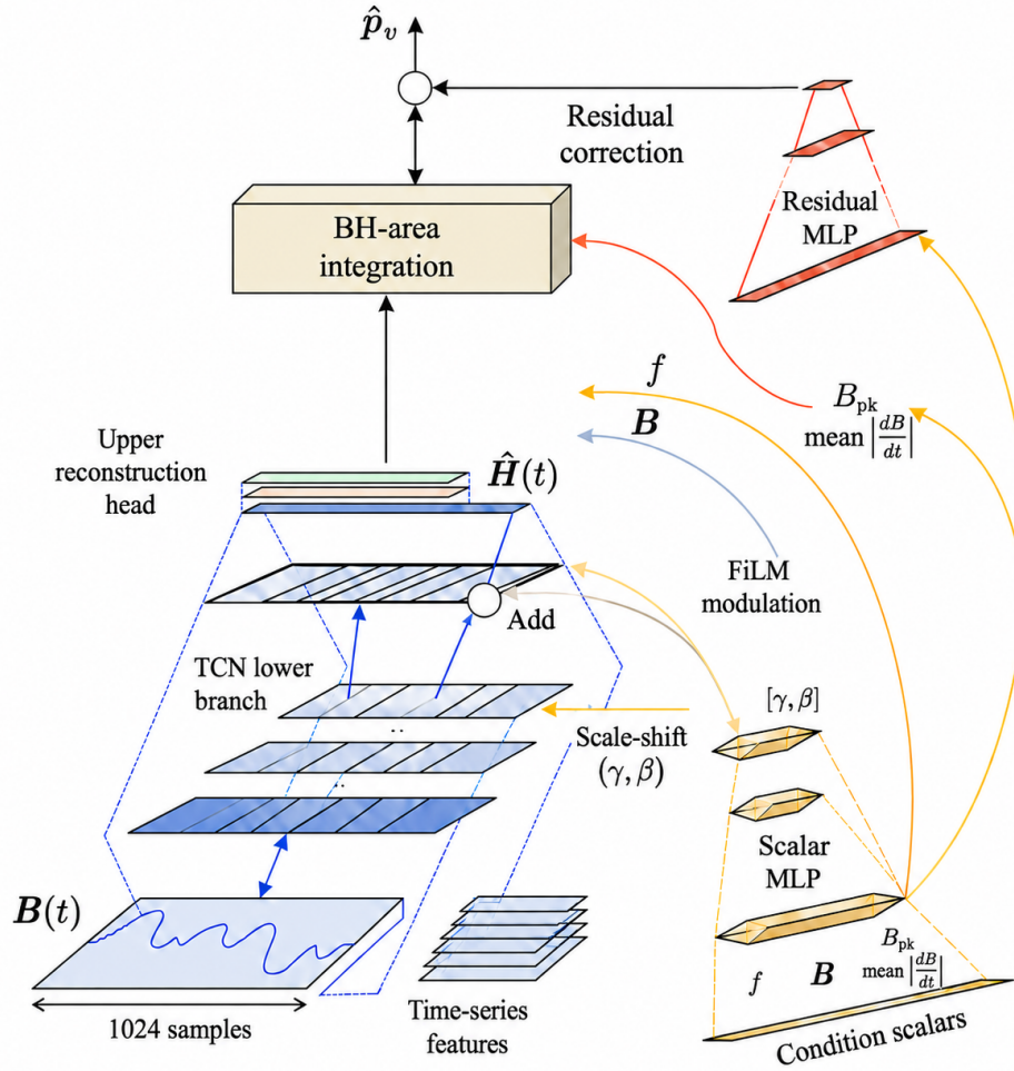
Fig. 1. Overall architecture of CAHR-Net. The operating vector \mathbf{s} is encoded into the FiLM pair [\gamma, \beta] , which rescales ( \odot , by 1 + \alpha\gamma ) and then shifts ( + , by \beta ) eleven of the twelve encoder channels before the magnetic-field reconstruction head; one raw channel bypasses modulation. The reconstructed field \hat{H}(t) drives the BH -area integration, and a residual multilayer perceptron corrects the loop-area estimate in the logarithmic loss domain to produce \hat{P}_v .
