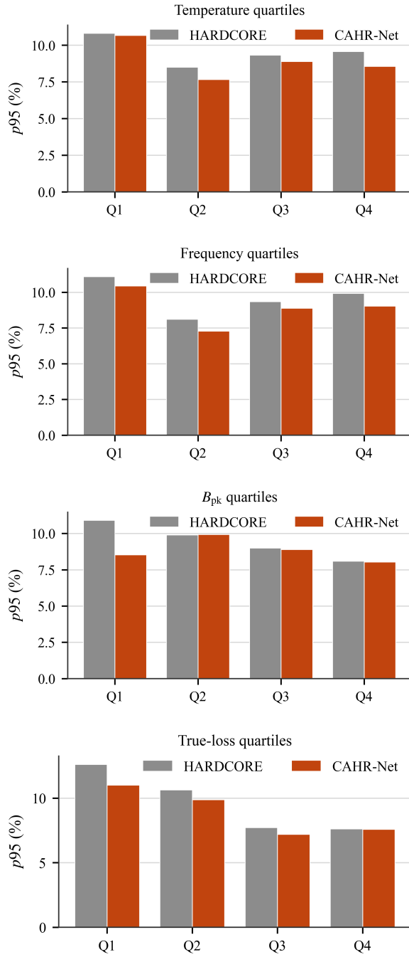
Fig. 5. Condition-slice analysis of p_{95} relative error, shown from top to bottom for temperature, frequency, peak flux density B_{pk} , and true loss magnitude quartiles.
