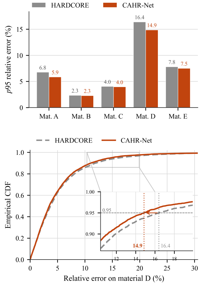
Fig. 4. Material-level tail analysis. (a) Material-level p_{95} comparison between HARDCORE and CAHR-Net. (b) Empirical cumulative distribution of relative error on material D; the inset magnifies the tail region around the 95th percentile, where CAHR-Net shifts the p_{95} from 16.40% to 14.87%.
