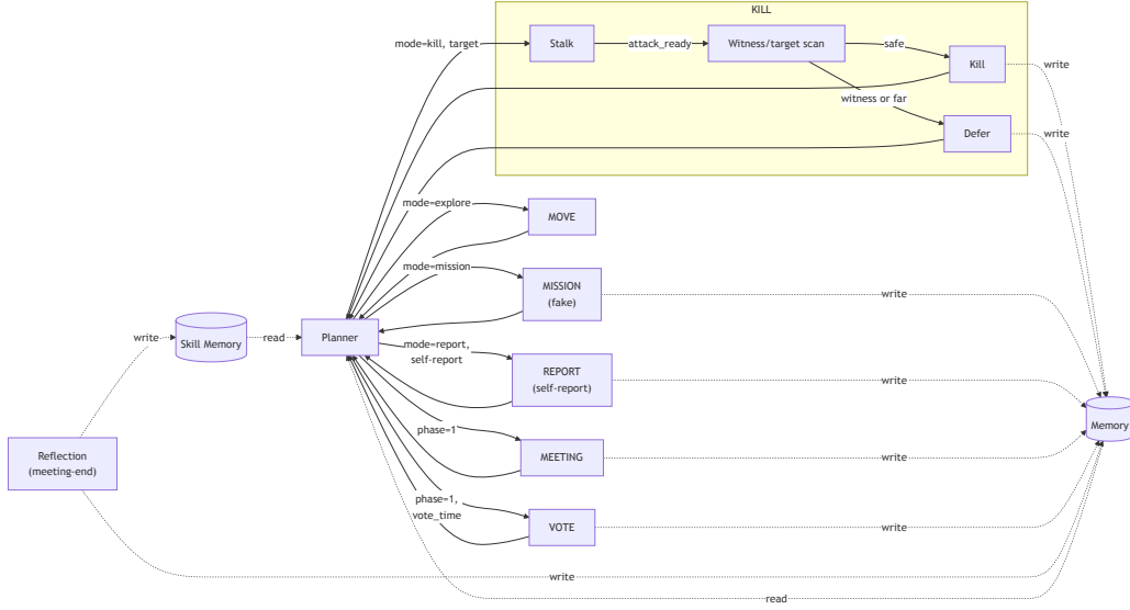
Figure 6: ARIA behavior cycle for imposter agents. The planner dispatches one of six task-phase modes; KILL runs as an internal stalk → witness/target scan → kill or defer state machine (sensorimotor pre-kill scan), MISSION is always fake-task cover, and REPORT doubles as self-report. During the meeting phase, the planner phase-forces MEETING or (during the voting window) VOTE. Memory and Skill Memory are read by the planner and written to by action modules; REFLECTION fires only at meeting-end and writes to both.
