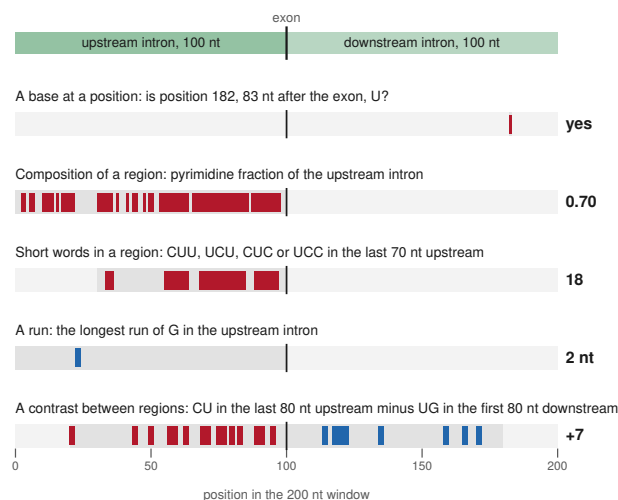
Figure 10 What a model is given, and the sparse linear model. a , Five features measured on one training exon of the PTBP1 task. The window is the two introns flanking the exon, joined. For each feature the grey band is the stretch it measures, the coloured cells are the bases it counts, and its value is given at the right. b , The ten-feature sparse linear model of the same task. Left, the weight of each feature, in log-odds per standard deviation of that feature. Right, the exon of panel a: its value on each feature, and what that adds to its score relative to an average training exon. Red argues silenced and blue enhanced, as in Fig. 5.
