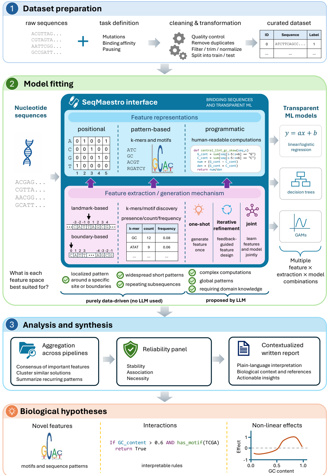
Figure 1 In this paper, we build a bridge between nucleotide sequences and interpretable machine learning.
