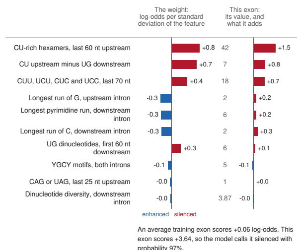
Figure 10 What a model is given, and the sparse linear model. a , Five features measured on one training exon of the PTBP1 task. The window is the two introns flanking the exon, joined. For each feature the grey band is the stretch it measures, the coloured cells are the bases it counts, and its value is given at the right. b , The ten-feature sparse linear model of the same task. Left, the weight of each feature, in log-odds per standard deviation of that feature. Right, the exon of panel a: its value on each feature, and what that adds to its score relative to an average training exon. Red argues silenced and blue enhanced, as in Fig. 5.
