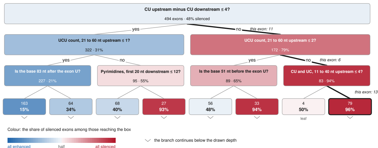
Figure 12 The decision tree. The ten-feature tree of the PTBP1 task with programmatic features written at each split, drawn to three levels. Each box gives the training exons that reach it and the share of them that are silenced, which also sets its colour, red for mostly silenced and blue for mostly enhanced. Chevrons mark branches that continue below the drawn depth. The heavy path is the route of the exon of Fig. 10a, with its values written on the edges.
