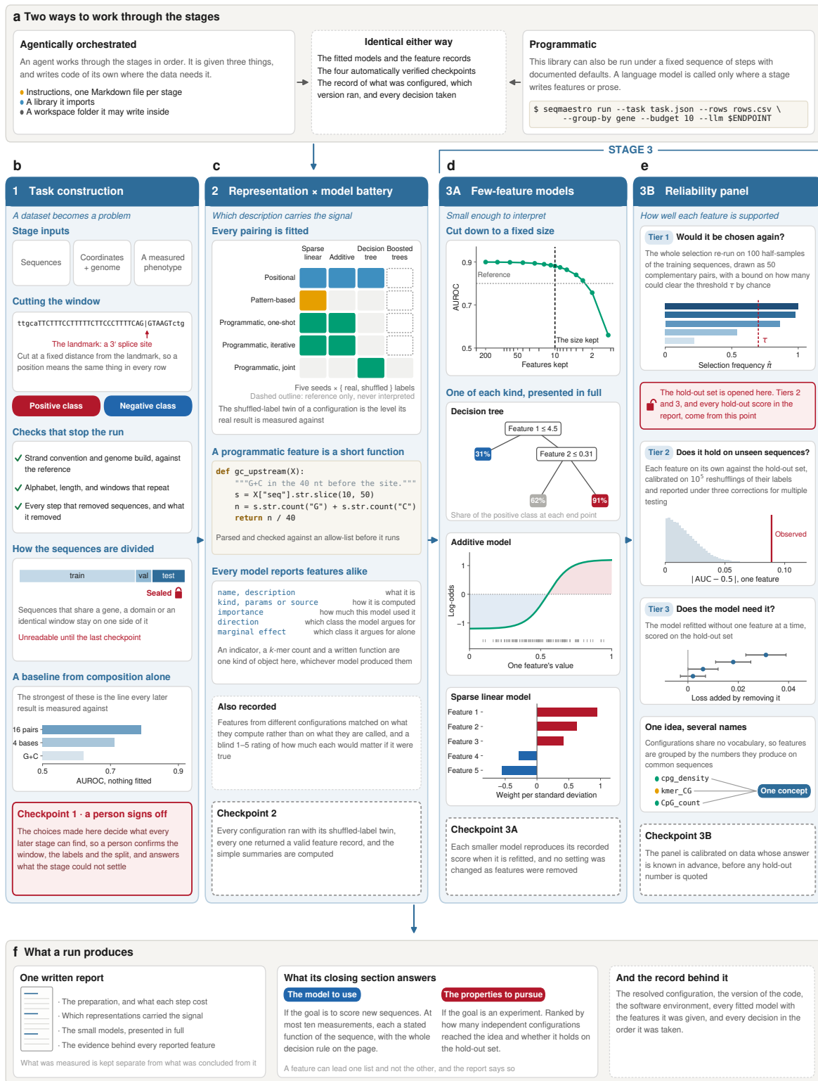
Figure 6 A SeqMaestro run. (a) The three stages are driven either by a tool-using AI agent, given written instructions for each stage, the SeqMaestro library, and a workspace folder, or run as a single command with sensible, documented defaults. Both routes follow these stages. (b) Stage 1 turns delivered data into a prediction problem, based on user interaction: the choice of sequence windows, and where they are aligned; provenance and composition of the data is checked; every filtered or discarded sequence is accounted for; and sequence stratification and grouping are defined. A simple composition-only model is recorded as a baseline. Finally, the user is asked to check and sign off this work at the checkpoint. (c) Stage 2 fits every pairing of a sequence feature representation with a compatible model, including a shuffled-label control. Key properties of discovered features are recorded in a standardized format. (d) Stage 3A reduces each configuration to a fixed number of features and records the best performing interpretable model of each kind. (e) Stage 3B evaluates every candidate feature whether the selection would return it on another half of the data, whether it separates the classes on unseen sequences, and whether the model loses accuracy when the feature is individually discarded. The hold-out set is opened the first of those three questions is settled. The other two (and every hold-out score in the report) are evaluated at the end. (f) A run produces a written report, which discusses both the best interpretable models, and the robust concepts/hypotheses discovered.
