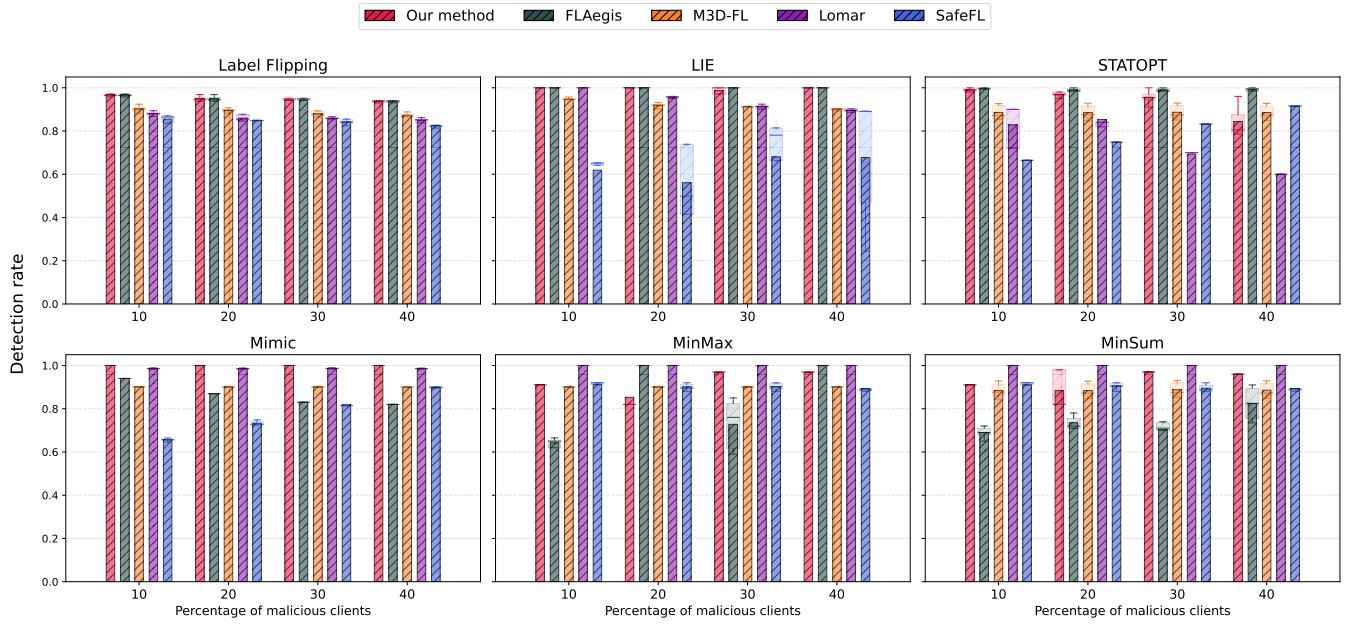
Figure 8: Detection accuracy of the different methods against the different poisoning attacks with different percentages with the sentiment140 dataset.
