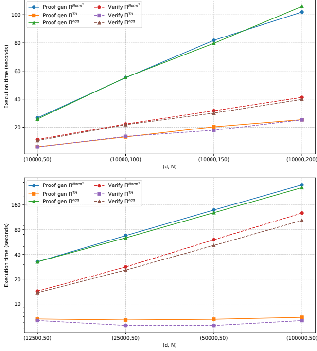
Figure 4: Proof generation and verification times for 4 sets of parameters with a fixed model dimension d (top) and a fixed number of clients N (bottom).
