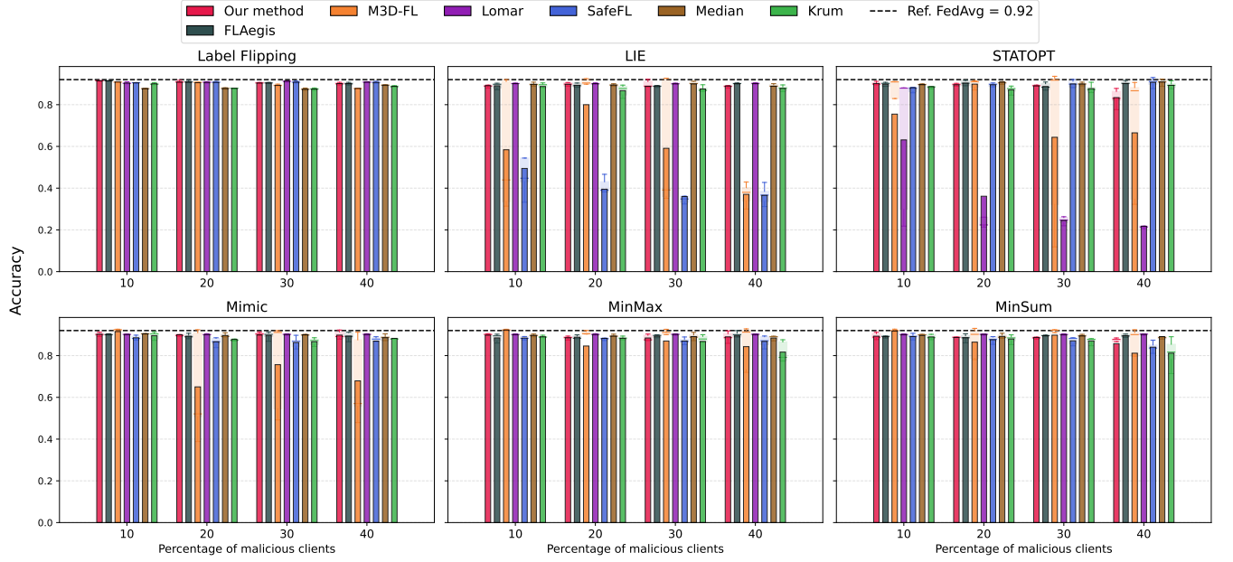
Figure 7: Final accuracy of the different methods against the different poisoning attacks with different percentages with the synthetic dataset.
