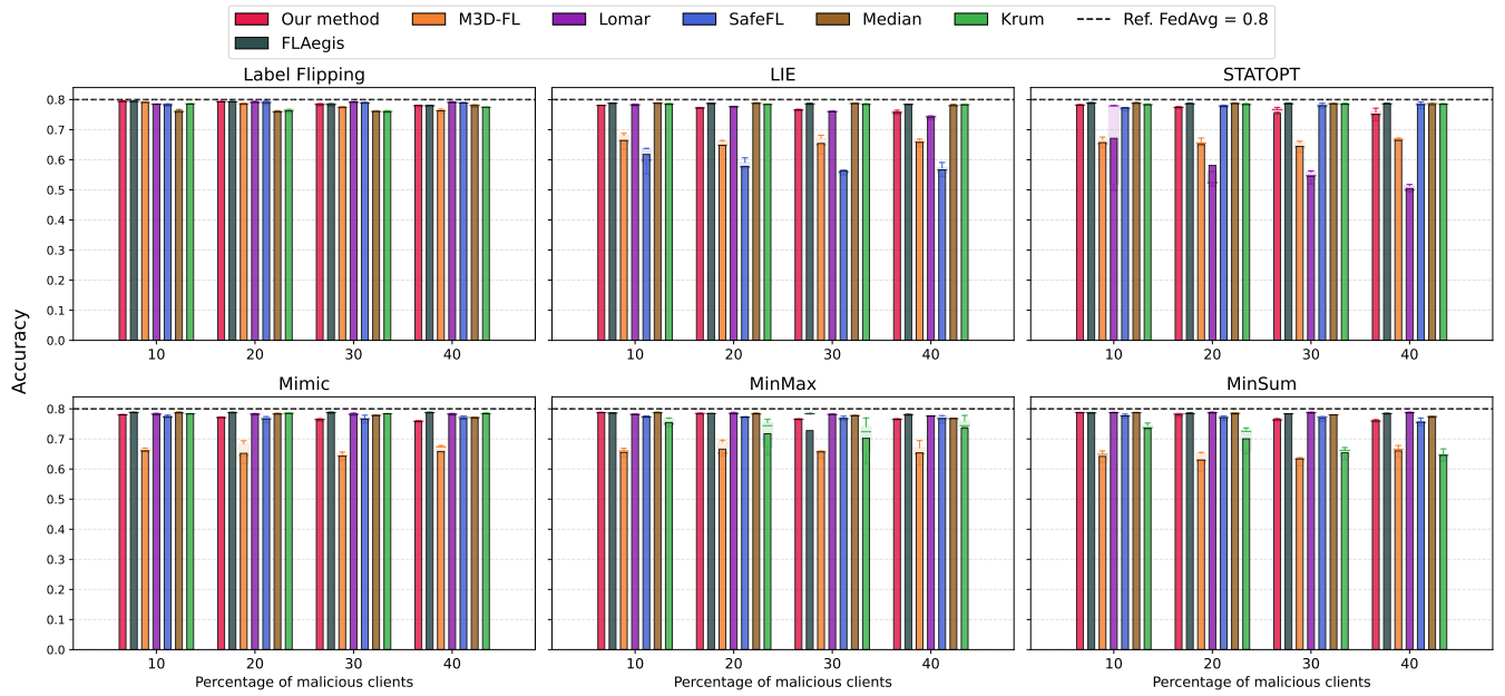
Figure 9: Final accuracy of the different methods against the different poisoning attacks with different percentages with the sentiment140 dataset.
