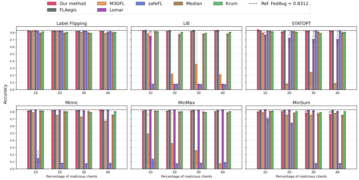
Figure 3: Final accuracy of the different methods against the different poisoning attacks with different percentages for FEMNIST dataset.
