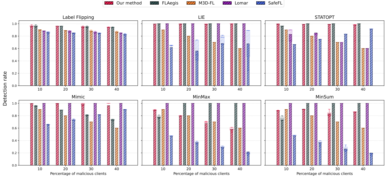
Figure 6: Detection accuracy of the different methods against the different poisoning attacks with different percentages with the synthetic dataset.
