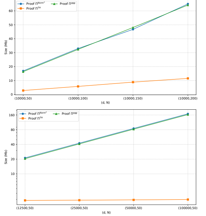
Figure 5: Proof size for 4 sets of parameters with a fixed model dimension d (top) and a fixed number of clients N (bottom).
