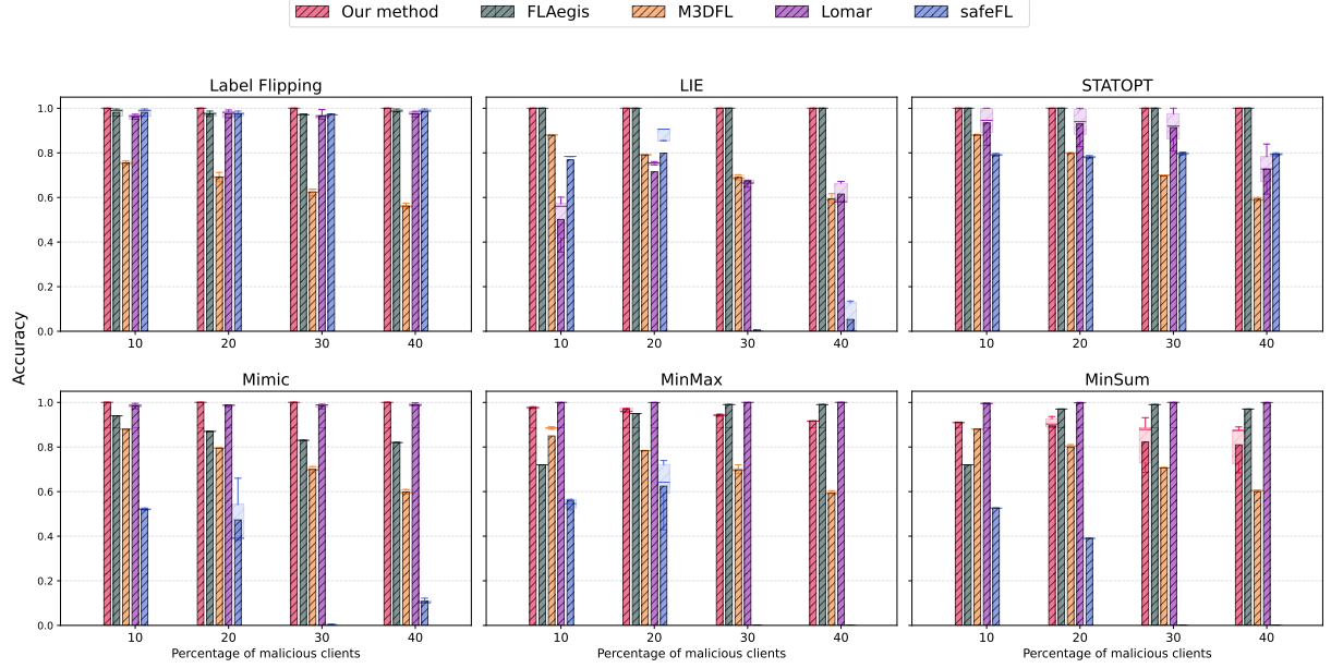
Figure 2: Detection accuracy of the different methods against the different poisoning attacks with different percentages for FEMNIST dataset.
