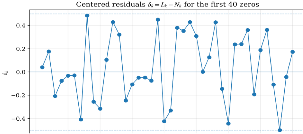
Figure 1: Centered residuals \delta_k = L_k - N_k for the first forty zeros. The interval [-1/2, 1/2] is intrinsic to nearest-integer centering. The visual absence of a simple trend motivates circular/Fourier diagnostics rather than ordinary linear regression.
