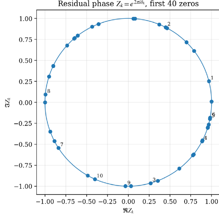
Figure 2: Unit-circle representation Z_k = e^{2\pi i \delta_k} for the first forty zeros. Labels 1–10 identify the first ten levels. Circularization removes the artificial discontinuity between residuals near +1/2 and -1/2 .
