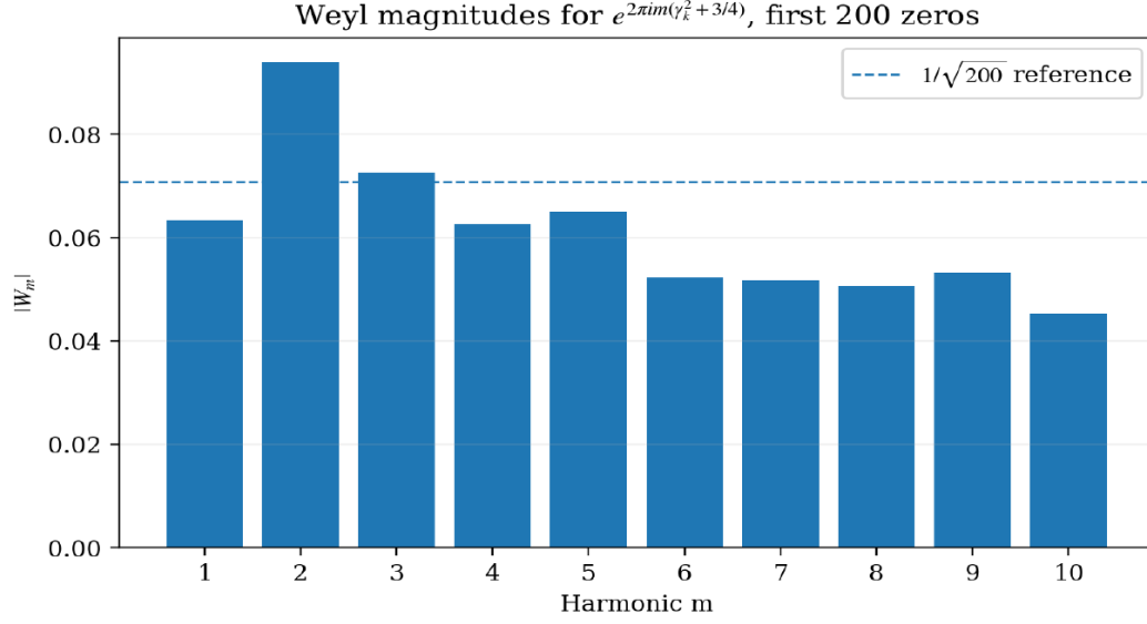
Figure 4: First ten Weyl magnitudes for e^{2\pi i m(\gamma_k^2 + 3/4)} , using the first 200 zeros. The dashed reference is 1/\sqrt{200} .
