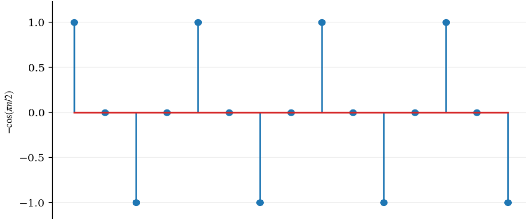
Figure 6: Exact sign/parity skeleton -\cos(\pi n/2) of the Bernoulli-number sequence for n \geq 2 .
