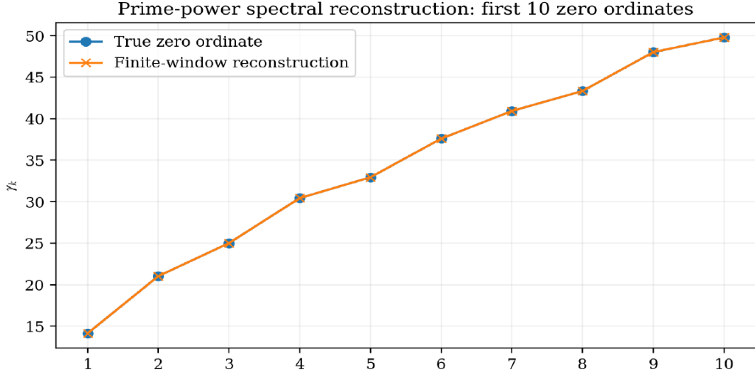
Figure 7: True versus finite-window reconstructed zero ordinates for k = 1, \dots, 10 . The curves nearly overlap for the early ordinates, while dL \approx 2\gamma d\gamma explains how a small ordinate error can become a much larger residual-phase error.
