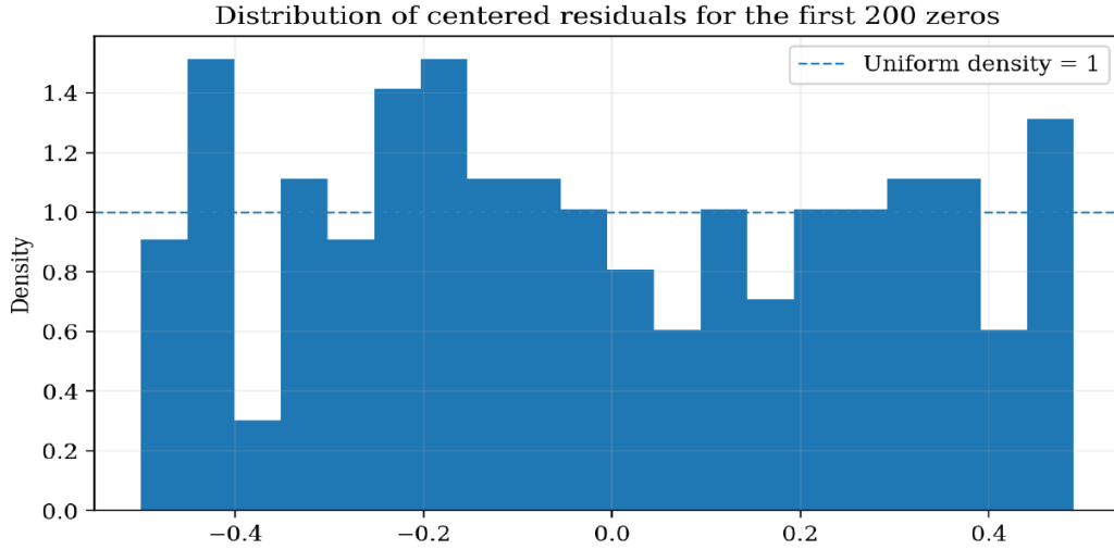
Figure 3: Histogram of the first 200 centered residuals. The dashed line is the density of U[-1/2, 1/2] . This is a finite-sample diagnostic only and does not establish equidistribution.
