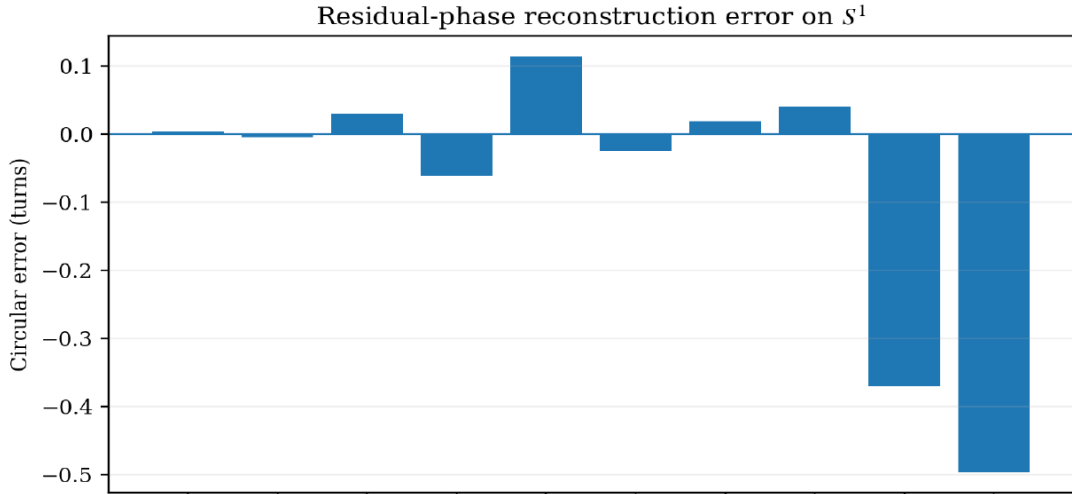
Figure 8: Circular reconstruction error measured in turns. The wraparound behavior illustrates why residual errors should be compared on S^1 rather than by ordinary subtraction near \pm 1/2 .
