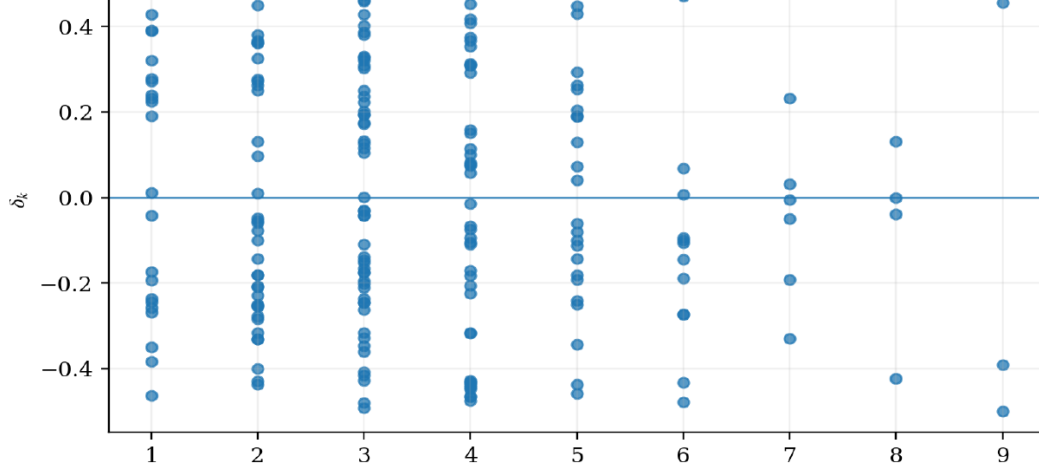
Figure 5: Residual versus total number of prime factors \Omega(N_k) for the first 200 levels. The scatter illustrates why a coarse factor-count statistic can discard too much of the prime-generator structure for a stronger shell-phase hypothesis.
