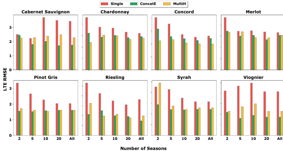
Fig. 3 We look at the cultivars with high amounts of data and artificially restrict the training set size for both the MTL and STL settings. We choose 2, 5, 10, 20, or all of the available seasons in the training set. The x-axis refers to the number of seasons included in the training set and the y-axis denotes the RMSE achieved. The complete set of results is included in Appendix B
