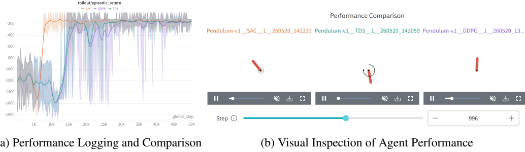
Figure 3: Logging of Deep RL Experiment Data. A further objective is to introduce students to deep RL workflows. The W&B integration allows managing large amounts of experiment data. Examples are (a) logging relevant quantities over several random seeds to compare algorithms or hyperparameter settings, and (b) recording videos of agent performance to inspect failure scenarios or connect a certain return value to the corresponding behavior.
