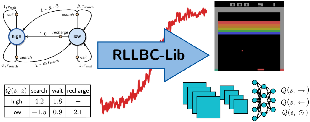
Figure 1: Didactic Concept of RLLBC-Lib. The presented code library lowers the entry barrier for students and other learners of RL. It starts from straightforward tabular settings, depicted on the left, to build a solid understanding of theoretical foundations. From there, it gradually guides towards state-of-the-art deep RL approaches, depicted on the right. This learning process is represented by the stylized return curve in red. The library builds on Jupyter notebooks with extensive explanations of theoretical concepts and their implementation. The notebook structure is consistent between tabular and deep RL approaches to underscore their similarities.
