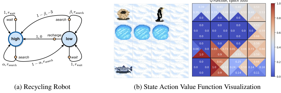
Figure 2: Examples of Illustrative Tabular Implementations. (a) Custom implementation of the recycling robot example in [34] to explain MDP dynamics and value functions. (b) Each state of the grid world is separated into triangles representing the action space \mathcal{A} = \{\leftarrow, \uparrow, \rightarrow, \downarrow\} . Plotting the state action values via color coding then illustrates learning dynamics.
